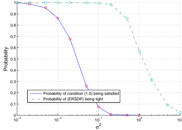
FIG. 2. Empirical probability of (ERSDP) being tight and condition (1.5) being satisfied.
