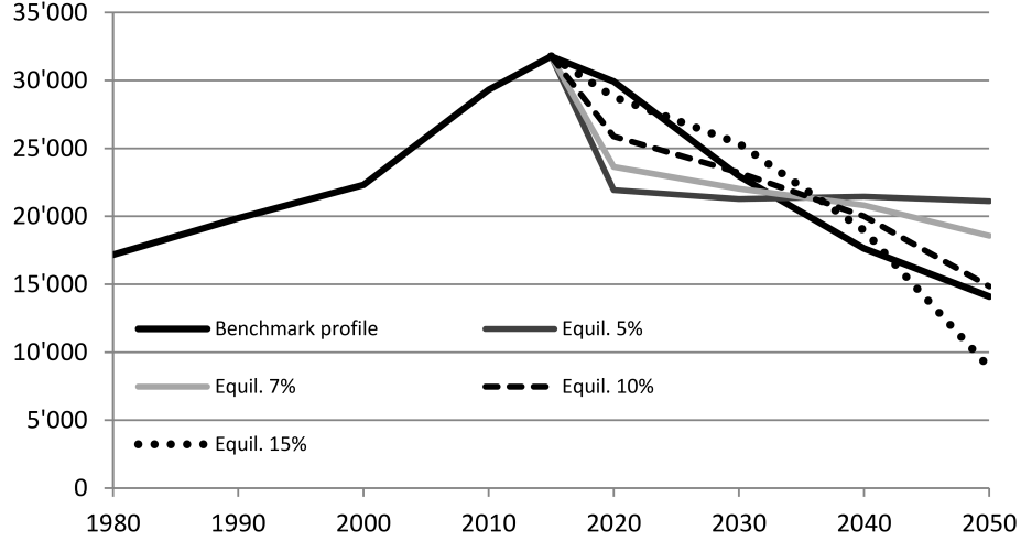
Figure 3: Emissions trajectory
