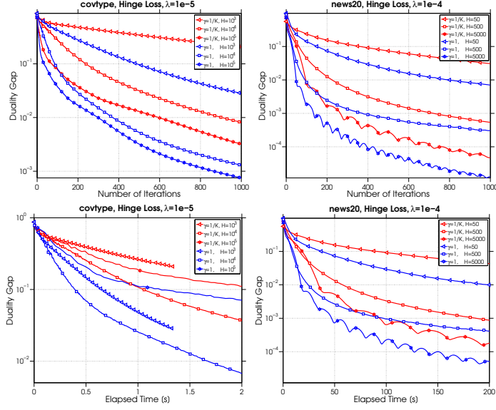
FIG. 4. Comparison of performance for different inner iteration limits when \sigma' = \frac{1}{K} and \sigma' = 1 .
