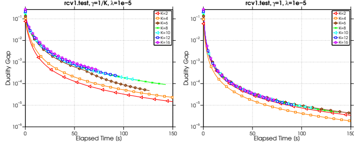
FIG. 6. Running times on different numbers of machines K .
