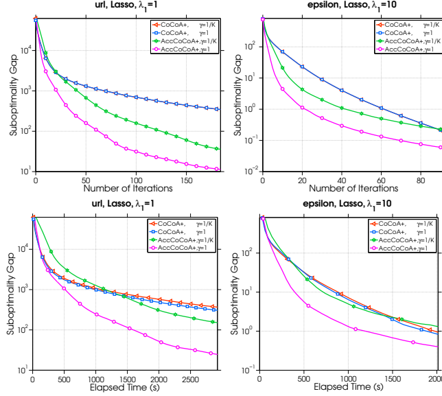
FIG. 3. Sub-optimality gap as a function of iterations (top row) and elapsed time (bottom row) when solving Lasso problems. The choice of the regularizer value ( \lambda_1 ) are such that for the url dataset the density of the optimal solution is 5.3%, while for the epsilon dataset the density is 13.56%.
