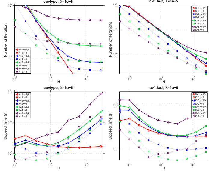
FIG. 5. Number of iterations and running time required to reach a tolerance of 10^{-3} on the duality gap as the inner iteration limit ( H ) is varied.
