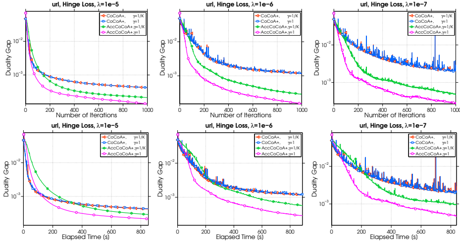
FIG. 2. Duality gap as a function of iterations (top row) and elapsed time (bottom row) when solving hinge-loss SVM problems with different regularization values ( \lambda ) on the url dataset.
