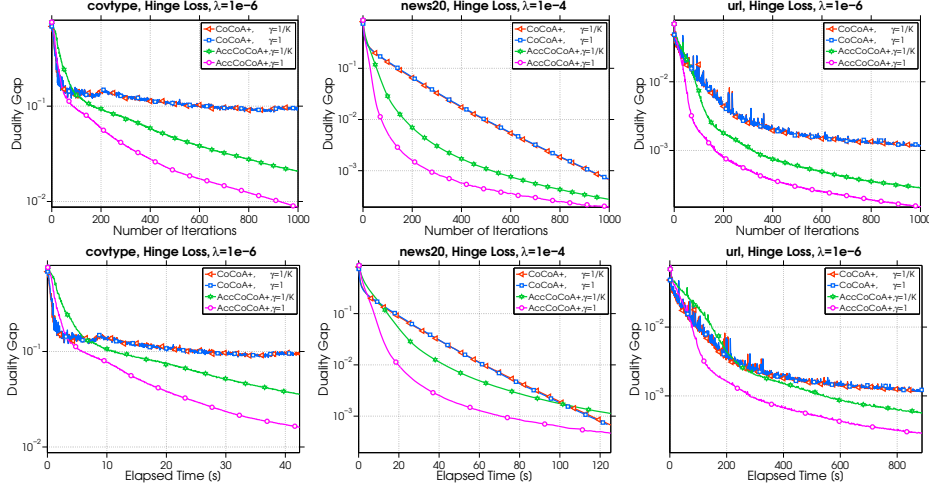
FIG. 1. Duality gap as a function of iterations (top row) and elapsed time (bottom row) when solving hinge-loss SVM problems.
