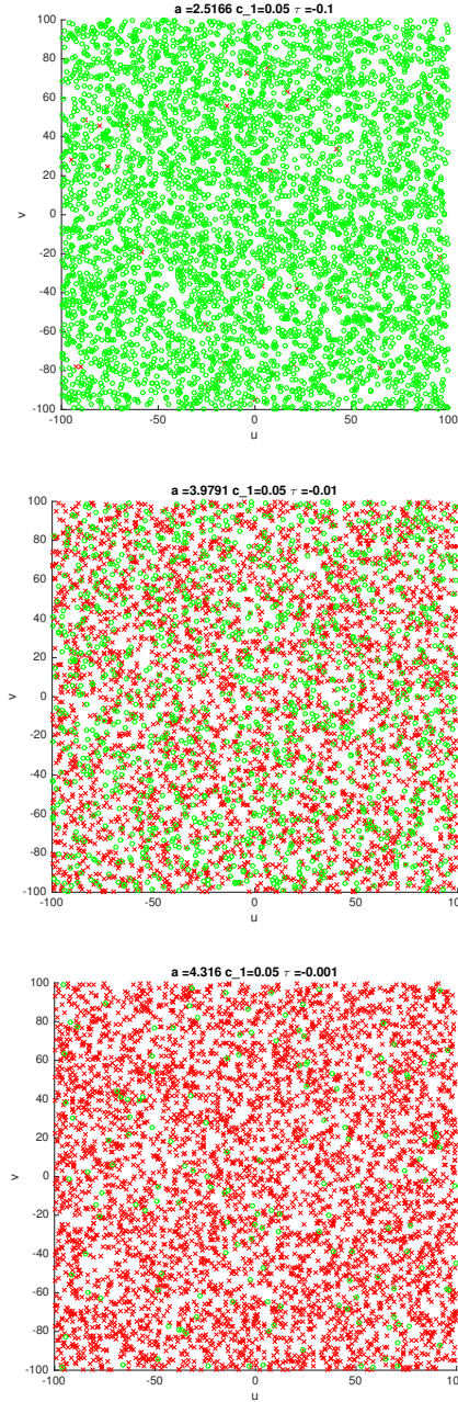
Figure 5: Mixed success and failure when \tau is negative but close to zero. Each plot shows 5000 points. The green circles show starting points for which the method succeeded, generating x_k = (u_k, v_k) \in \mathbb{R}^2 for which f(x_k) is apparently unbounded below, while the red crosses show starting points for which the method failed, generating x_k converging to a point on the v -axis.
