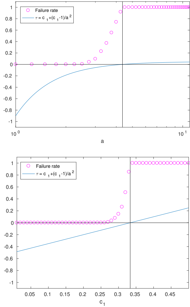
Figure 4: Failure rates (small circles) for f with n = 2 when (top) c_1 is fixed to 0.05 and a is varied and (bottom) a is fixed to \sqrt{2} and c_1 is varied. The solid curves show the value of \tau . Each experiment was repeated 5000 times.
