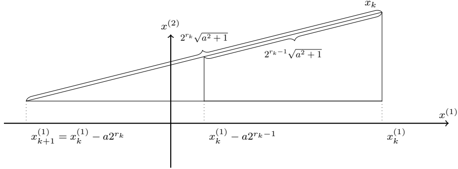
Figure 1: Doubling t in order to satisfy W(t) .
