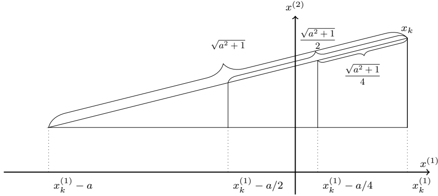
Figure 2: Halving t in order to satisfy A(t) .
