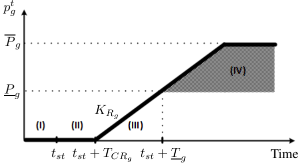
(b) The first part of the decomposed generator model. The generation levels in the graph are defined as \underline{P}_g = P_g^{\min} + P_{CR_g} and \bar{P}_g = P_g^{\max} + P_{CR_g} .
