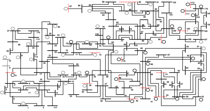
Fig. 6: Snapshot of the IEEE-118 system ( t = 10 ). The non energized part is depicted in gray, generators with bold black line have nonzero output, whereas dotted generators are being cranked. Red dotted bus lines and red dashed bus lines indicate buses at their maximum and minimum voltage respectively. Note that buses of generators with reactive power support (such as 46) are usually set to the minimum voltage (in order to absorb reactive power), whereas some buses at the edges of transmission (such as 51) are set to the maximum.
