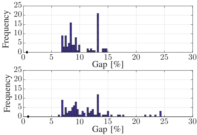
Fig. 5: Gap for 100 feasible solutions generated by the heuristic, for two different settings of the value of \alpha_{BS} , i.e. \alpha_{BS} = 0 (plot above) and \alpha_{BS} = 1.5 (plot below). The values of \alpha_E and \alpha_G are set to 0.5. The heuristic solutions were fed to the optimizer, which solved the problem within 1% tolerance. The gap for that solution is shown with a diamond on the plots. Increased randomness (meaning the heuristic moves randomly away from the LP relaxation solution) leads to worse feasible solutions in general, but may also get lucky and find a better feasible solution.
