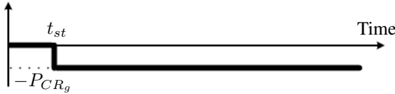
(c) The second part of the decomposed generator model. This is essentially a negative step function to the cranking power of the generating unit at the time of energization ( u_g^t = 1 ). The allocation of the BS units allows for u_g^t to become 1, even if there is no external power fed to the unit.
