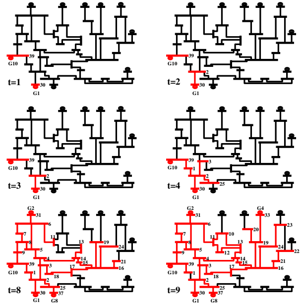
Fig. 3: Sampled steps of the restoration process. Generators 1 and 10 are chosen by the optimization problem as BS units, so they get energized first. The rest of the grid is gradually restored. The time unit is 5min. Note that the line connecting buses 2 and 30 is picked up immediately after energization, because it has no shunt capacitance in the model. However, the generators cannot pick further transmission lines immediately, since they can not change their reactive power setpoint up until one period after the cranking is over (i.e. after time 3 for G1). Notice also that the line connecting buses 1 and 39 gets de-energized at time t = 9 . Forcing energization of the line at this time point leads to ac infeasibility, which means that the flexibility of de-energizing lines (enabled by the model) is utilized.
