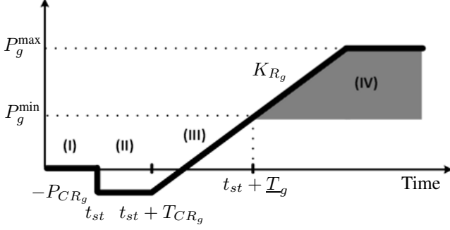
(a) A disconnected generator g \in G (phase I) gets energized at time t_{st} (i.e. u_g^t becomes 1 at t = t_{st} ) and needs to be cranked for a period of T_{CR_g} (phase II). During the cranking period, the generator absorbs the cranking power P_{CR_g} . (negative generation). The generator then starts to ramp up to its technical minimum \underline{P}_g (phase III) at time t_{st} + T_g , where T_g = T_{CR_g} + (P_{CR_g} + P_g^{\min}) / K_{R_g} . Afterwards, generation can freely move between P_g^{\min} and P_g^{\max} , within the ramping capability K_{R_g} . This model appears in other works, such as in [8] and [11]. For the purposes of this work, we decompose the model as the superposition of the two curves below.
