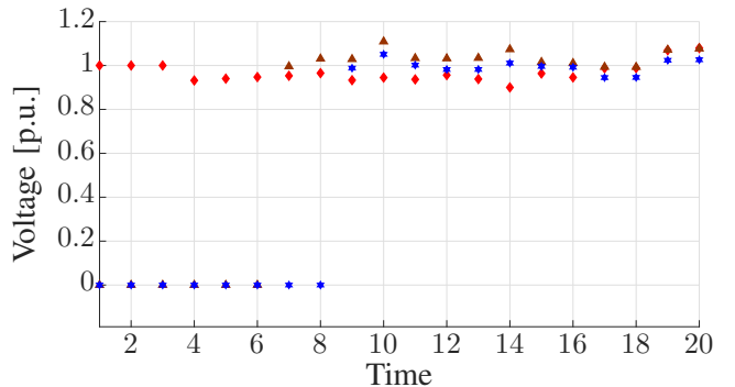
Fig. 4: Voltages of three buses from the ac simulations. Bus 16 (brown triangles) is on the edges of the transmission system and suffers from overvoltages (in fact at time t = 10 we need to relax the voltage limit to 1.12p.u. for one time step). Bus 30 (red diamonds) is a generator bus and its value is set as low as possible, to accommodate for reactive power transfer to the transmission system. Finally, the voltage of bus 20 is depicted with blue hexagrams. The transition from zero to nonzero values indicates the time step that a node is energized.
