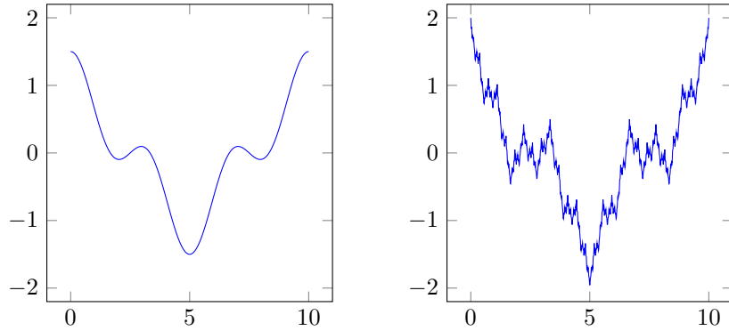
Figure 3: Approximants of the Weierstraß function by including one summand (left) and ten summands (right).
