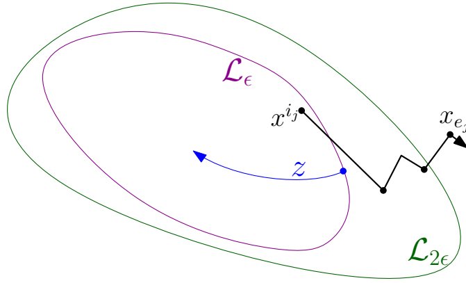
Figure 1: Illustration of the non-escape argument
