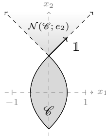
FIGURE 1. The set \mathcal{C} defined in (76) and its normal cone \mathcal{N}(\mathcal{C}; e_2) at e_2 .
