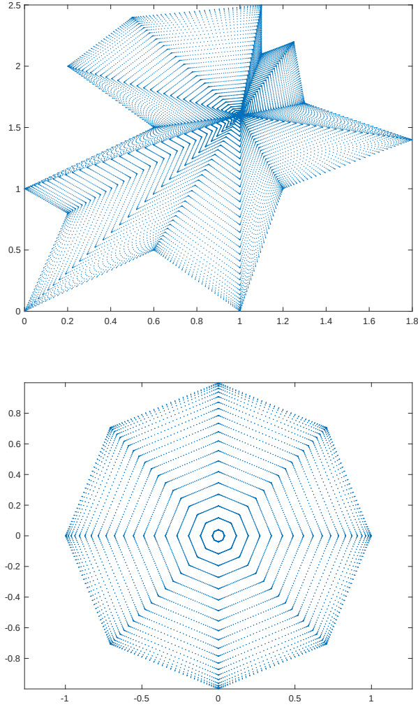
Figure 1: Chebyshev-Dubiner webs for polynomial minimization of degree n = 4 with a range-relative error less than 5%, on a 14-side starlike polygon (around 21000 points) and on a regular octagon (around 7700 points).
