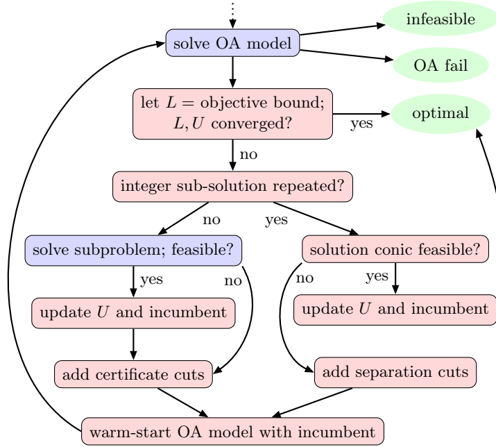
Figure 3: Pajarito's iterative method, following initialization.
