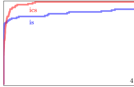
(b) MSD - execution time.
