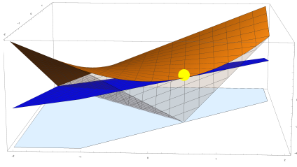
(a) Improving separation: Two functions that are valid underestimators for x_i x_j (orange) on a polyhedral domain (cyan). The figure shows that a linearization of the convex envelope (blue) at a given point (yellow) is locally tighter than the McCormick relaxation (gray).
