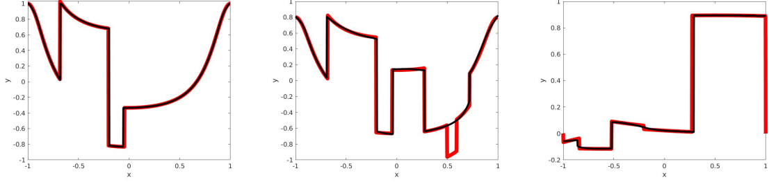
Figure 5: Degree 10 semi-algebraic approximations (black) for the discontinuous univariate functions (red) of Examples 65 (left), 66 (middle) and 67 (right) of reference [11].
