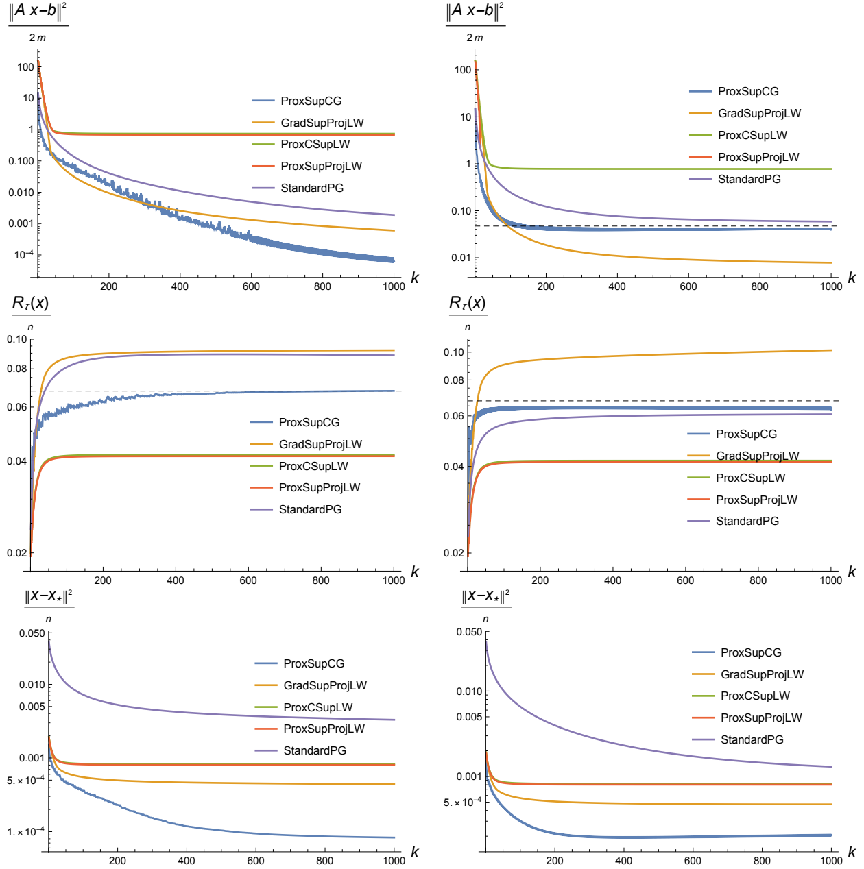
FIGURE 6.5. Superiorization: Adding Nonnegative Constraints. Scaled values of the data term (top row) and the regularizer (middle row) of the objective (1.2) and the squared error norm (bottom row), as a function of the iterative steps k of the superiorized CG iteration (4.20) and the Landweber iteration (4.21) using proximal points, see (4.18), the gradient and proximal-point based superiorized projected Landweber iteration and the FB iteration (5.58) for the reversed splitting. The dashed lines in the middle row plots indicate the corresponding values for x_* . The left and right columns correspond to exact and noisy data, respectively. Constraints are incorporated either in the basic algorithm (GradSupProjLW, ProxSupProjLW) or via the superiorization strategy (ProxCSupCG, ProxCSupLW) by constraining proximal points. Superiorized versions of the Landweber iteration perform similarly making slow progress towards x_* due to the bad conditioning of A , with a surprising better performance of the gradient based superiorized projected Landweber iteration GradSupProjLW. Again, the superiorized CG iteration approaches the solution of (1.2) significantly faster than the FB iteration (5.58) after appropriate parameter tuning.
