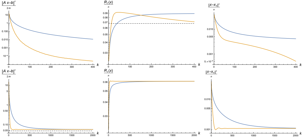
FIGURE 6.8. Optimization: FB and accelerated FB iteration for the reversed splitting – Nonnegativity Constraints. Scaled values of the data term (left column) and the regularizer (center column) of the nonnegatively constrained objective (1.2) and the squared error norm (right column), as a function of the iterative steps k of the FB iteration (5.58) (dark curves) and the accelerated FB iteration (5.59) for the reversed splitting. The dashed lines indicate the corresponding values for x_* . The top and bottom row correspond to exact and noisy data. While the FB iteration is damped by the inclusion of constraints, the nonnegativity constraints appear to be beneficial for the accelerated FB iteration on the other hand when comparing to the results from Figure 6.7.
