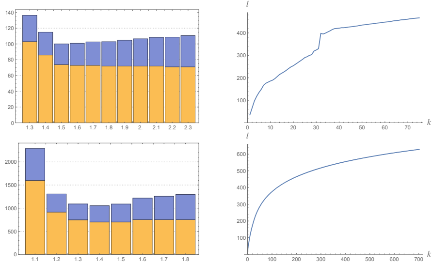
FIGURE 6.10. Inexact accelerated FB iteration for the nonnegatively constrained problem (1.2). LEFT: Relation of the number of outer iterations (not scaled down) and the total number of inner iterations (scaled down by 1/1000) as a function of the exponent q of the error \varepsilon_k = \mathcal{O}(k^{-q}) (5.23). RIGHT: Number \ell of inner iterations at each outer iteration k , for exponents q = 1.8 (top) and q = 2.0 (bottom) of (5.23).
