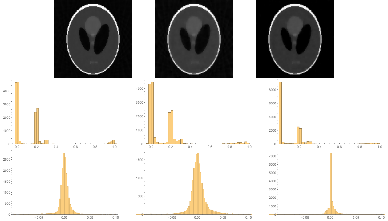
FIGURE 6.3. TOP ROW, FROM LEFT TO RIGHT: Minimizers x of the unconstrained objective function (1.2) for exact data, for noisy data, and minimizer for the nonnegatively constrained objective function and noisy data. CENTER ROW: The histograms corresponding to the top row. In the unconstrained cases, a number of components x_i are outside the range [0, 1] of x_*, i \in [n] . BOTTOM ROW: The difference histograms of x - x_* corresponding to the top row. The left histogram (unconstrained case, exact data) peaks more sharply around 0 than the histogram in the center (unconstrained case, noisy data), and significantly so on the right (nonnegatively constrained case, noisy data).
