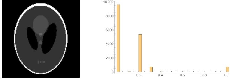
FIGURE 6.1. LEFT: The original image x_* of size n = 128^2 to be recovered from m = 0.15625n linear measurements. Both exact and noisy measurements are considered. RIGHT: The histogram of the original image x_* that plots the number of pixels for each intensity value.
