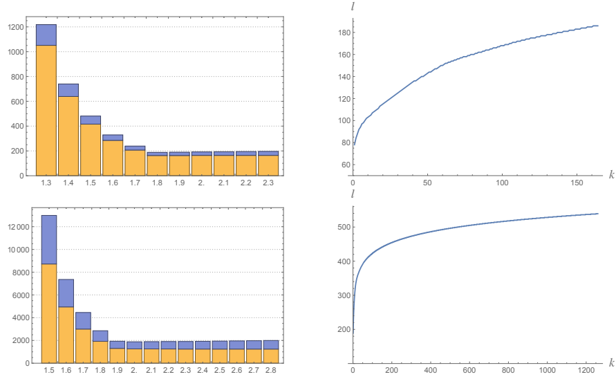
FIGURE 6.9. Inexact accelerated FB iteration for the unconstrained problem (1.2). LEFT: Relation of the number of outer iterations (not scaled down) and the total number of inner iterations (scaled down by 1/1000) as a function of the exponent q of the error \varepsilon_k = \mathcal{O}(k^{-q}) (5.23). RIGHT: Number \ell of inner iterations at each outer iteration k , for exponents q = 1.8 (top) and q = 2.0 (bottom) of (5.23).
