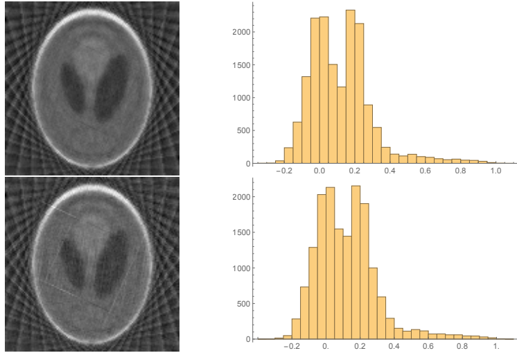
FIGURE 6.2. Regularized least-squares solutions determined by (6.3) for exact b (top) and for noisy b (bottom) illustrate the ill-posedness of the problem to recover the data shown by Figure 6.1 from m = 0.15625n linear measurements comprising the data vector b .
