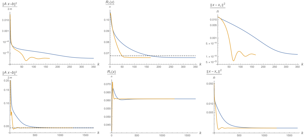
FIGURE 6.6. Optimization: FB and accelerated FB iteration – No Constraints. Scaled values of the data term (left column) and the regularizer (center column) of the objective (1.2) and the squared error norm (right column), as a function of the iterative steps k of the FB iteration (5.13) (dark curves) and the accelerated FB iteration (5.22). The dashed lines indicate the corresponding values for x_* . The top and bottom row correspond to exact and noisy data: accelerated FB needs about 50% and 25% less outer iterations, respectively.
