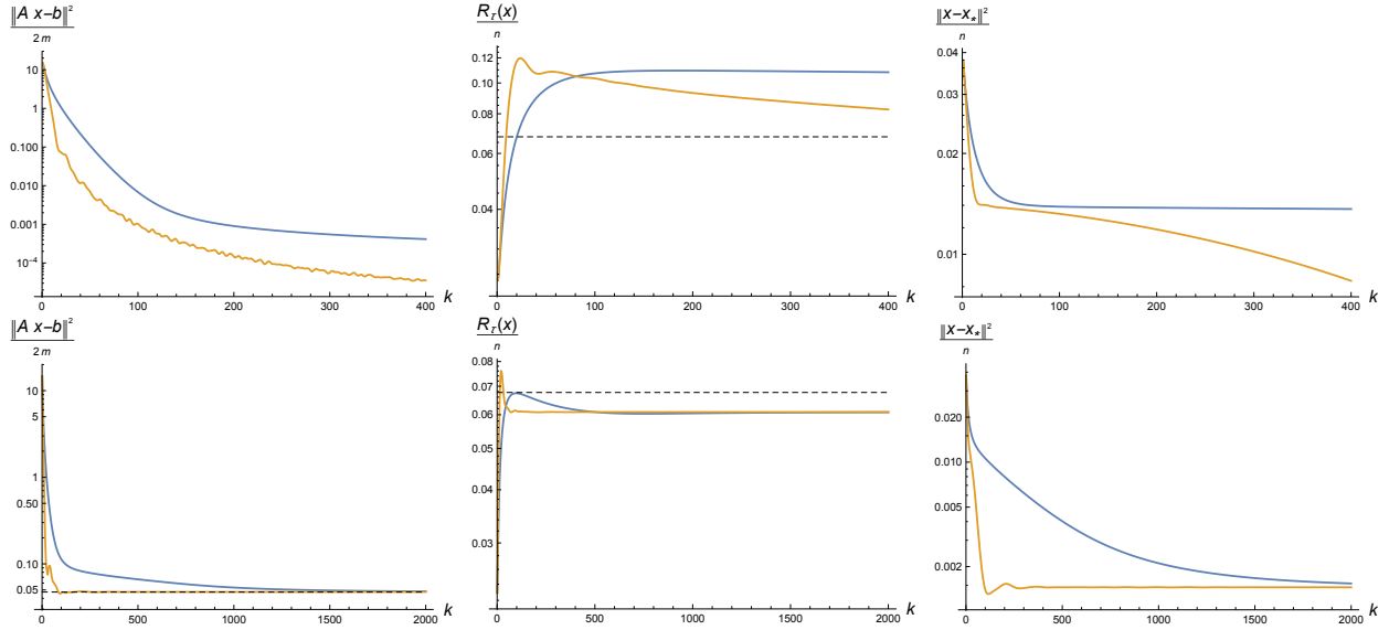
FIGURE 6.7. Optimization: FB and accelerated FB iteration for the reversed splitting – No Constraints. Scaled values of the data term (left column) and the regularizer (center column) of the unconstrained objective (1.2) and the squared error norm (right column), as a function of the iterative steps k of the FB iteration (5.58) (dark curves) and the accelerated FB iteration (5.59) for the reversed splitting. The dashed lines indicate the corresponding values for x_* . The top and bottom row correspond to exact and noisy data.
