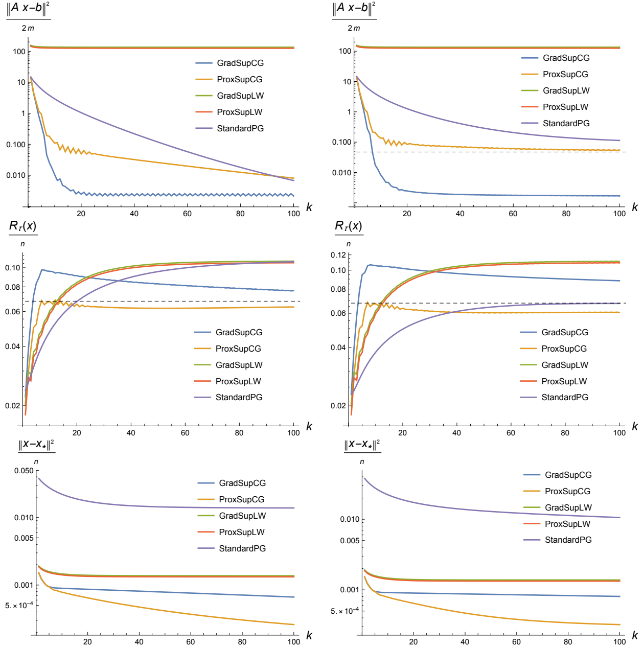
FIGURE 6.4. Superiorization: Unconstrained Least-Squares. Scaled values of the data term (top row) and the regularizer (middle row) of the objective (1.2) and the squared error norm (bottom row), as a function of the iterative steps k of the superiorized CG iteration using both perturbations based on gradients, see Algorithm 3 and proximal points, see (4.16), the gradient and proximal-point based superiorized Landweber iteration and the FB iteration (5.58) for the reversed splitting. The dashed lines in the middle of the plots indicate the corresponding values for x_* . The left and right columns correspond to exact and noisy data. Both the basic algorithm and the superiorization strategy does not incorporate nonnegativity constraints, respectively. After appropriate parameter tuning the Superiorized CG iteration approaches the solution of (1.2) significantly faster than the FB iteration (5.58). The superiorized Landweber iteration makes slow progress due to very small step-sizes in view of the large value of \|A\|^2 .
