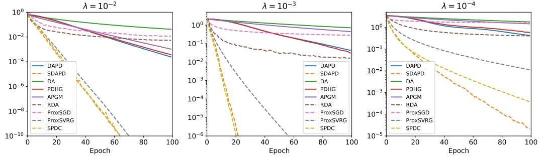
Figure 1. Comparison on synthetic data with different choices of \lambda . The y -axis is the primal sub-optimality, namely P(x^t) - P(x^*) . The solid lines are deterministic methods, and the dashed lines stand for stochastic methods. Here an epoch refers to one iteration for deterministic methods, and n times accesses to the vectors a_i for stochastic methods.
