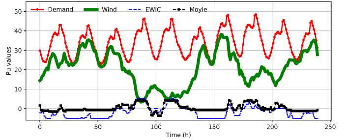
Fig. 5. Demand, wind and import/export variation with time
