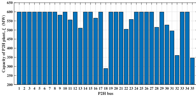
Fig. 7. Impact of P2H plant location on its optimal capacity
