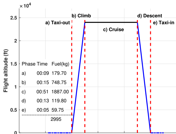
Fig. 3. Fuel consumption in each flight phase for DUB-LHR route
