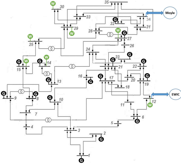
Fig. 4. Irish representative transmission network
