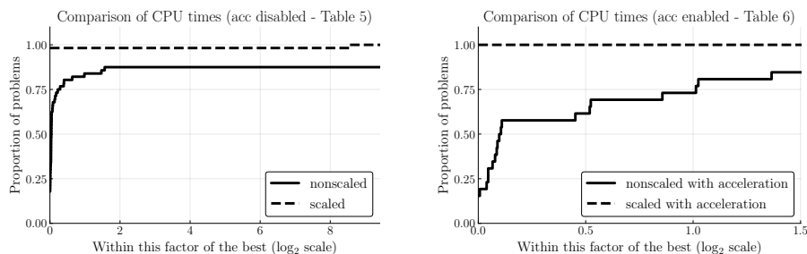
Fig. 1 Visual representation of the data of Tables 5 and 6, emphasizing the problems where the nonscaled and scaled variants performed differently.
