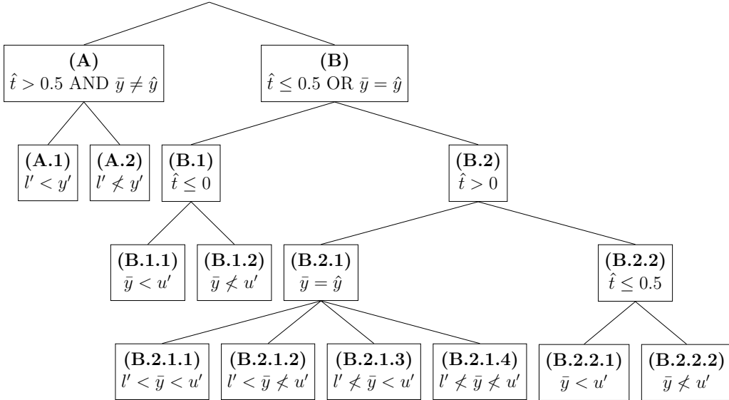
Figure 7: Case distinction for Theorem 4.2
