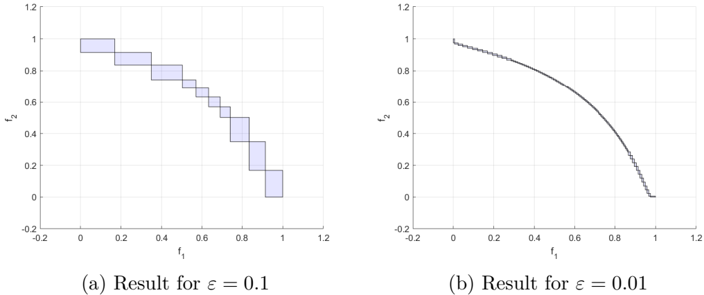
Figure 11: Numerical results for (MOP2)
