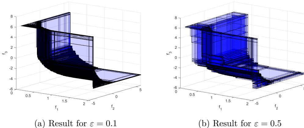
Figure 10: Numerical results for (Ex5.1)
