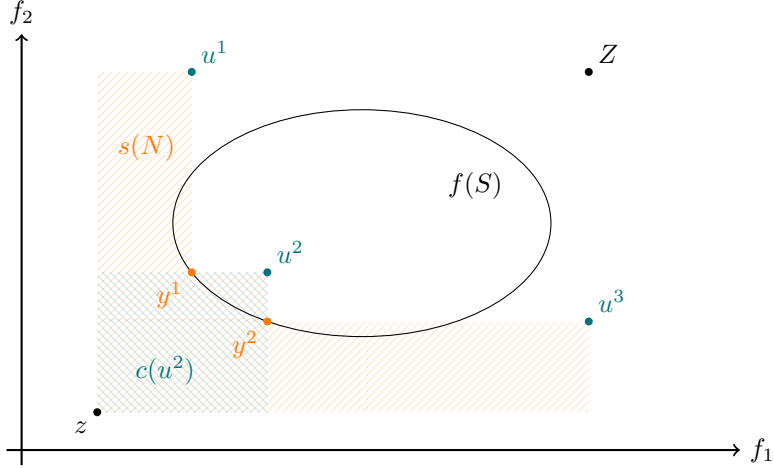
Figure 2: Illustration of lower search region, lower search zone and local upper bounds
