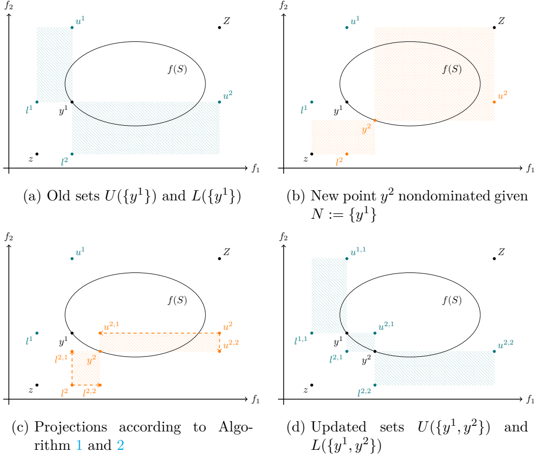
Figure 4: Illustration of update procedure based on Algorithm 1 and Algorithm 2
