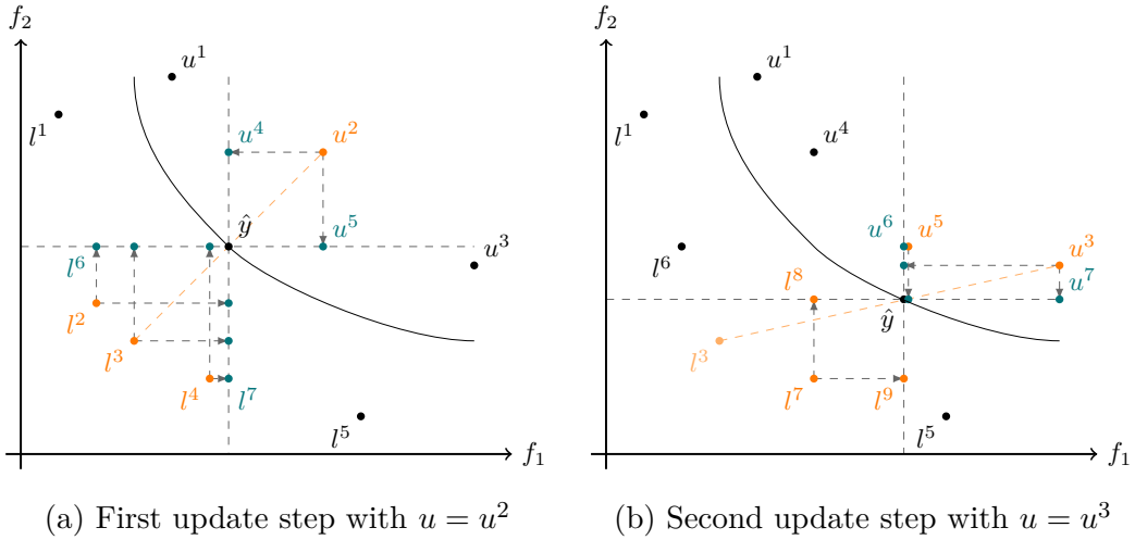
Figure 6: Two subsequent update steps from Algorithm 3 with l = l^3
