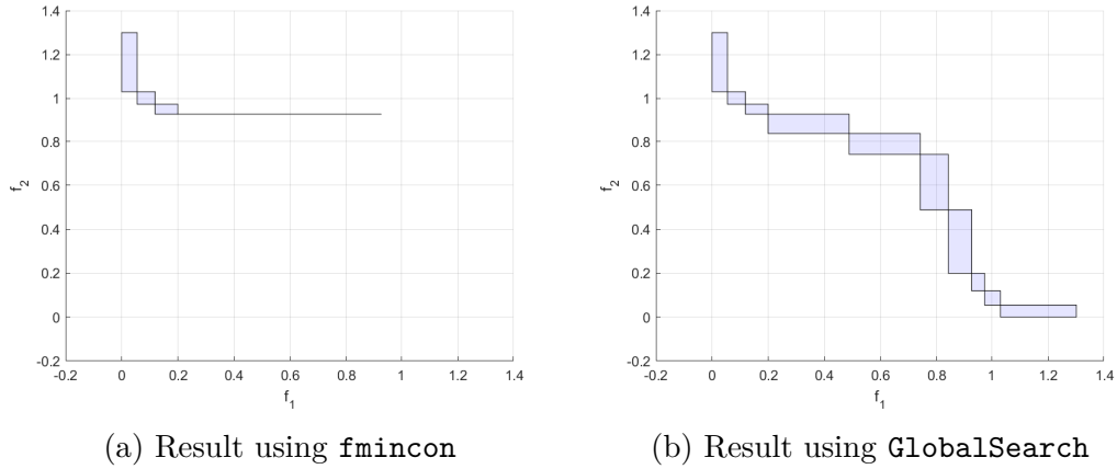
Figure 12: Numerical results for (Tan)
