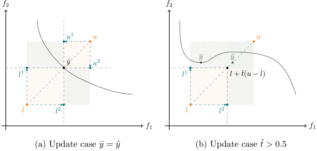
Figure 5: Two update scenarios from Algorithm 3
