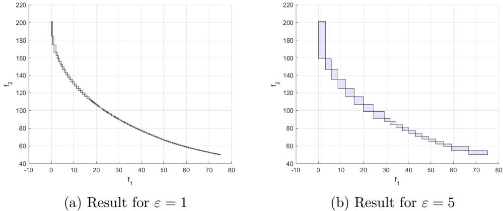
Figure 8: Numerical results for (Br)
