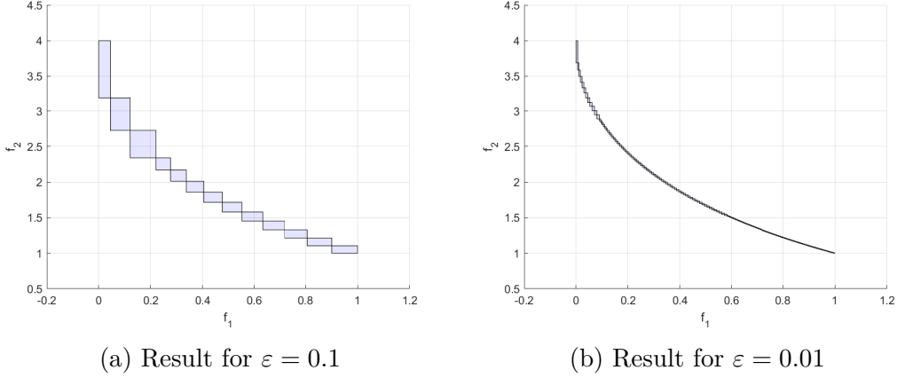
Figure 9: Numerical results for (Jin1)
