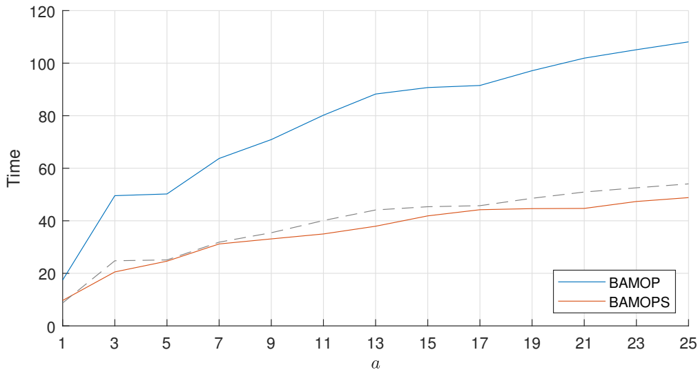
Figure 13: Comparison of BAMOP and BAMOPS for (Ex5.1)
