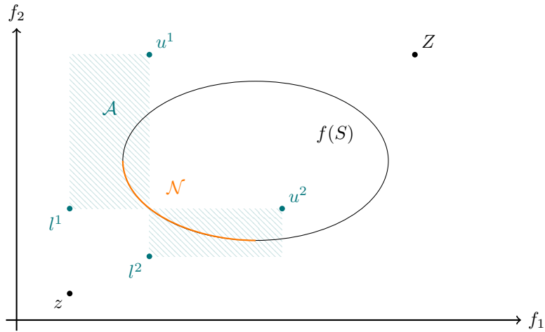
Figure 1: Illustration of approximation \mathcal{A} for L = \{l^1, l^2\} and U = \{u^1, u^2\}
