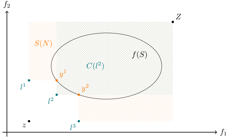
Figure 3: Illustration of upper search region, upper search zone and local lower bounds
