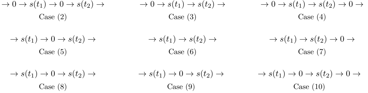
Figure 3: Possible cases for the costs associated with variables y_{t_1, j_1, t_2, j_2} .
