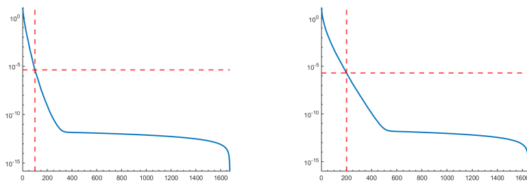
Fig. 2: \Sigma(r) over r = 1, \dots, \tilde{N} - 1 for the Poisson (left) and the convection-diffusion (right) problem. Red dotted lines indicate the chosen reduced dimensions for the later numerical experiments.
