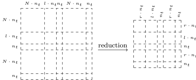
Fig. 1: Schematic dimension reduction from the Newton equation with \mathcal{N} in (30) to the reduced one with \mathcal{N}_{\text{red}} in (29) obtained via balanced truncation.
