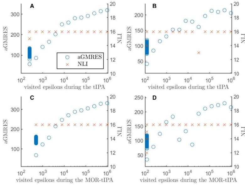
Fig. 3: Number of outer IPM iterations (right y-axis) and average GMRES iterations (left y-axis) during the tIPA for the Poisson (A) and convection-diffusion (B) problem as well as the MOR-tIPA for the Poisson (C) and convection-diffusion (D) problem.
