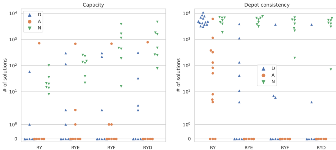
Figure 7: Numbers of infeasible solutions violating capacity and depot-consistency requirements.
