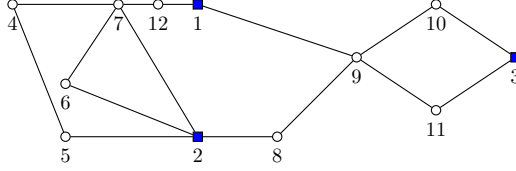
Figure 12: A candidate solution which is infeasible for the MDSDVRP which violates multi-leg PE constraints (10), but satisfies those considering at most two legs.
