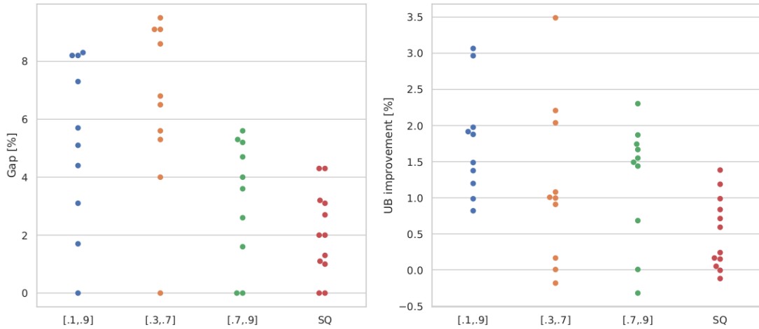
Figure 10: Optimality gaps [%] and improvements of upper bounds [%] over previously best known [25] of branch-and-cut for the MDS DVRP.
