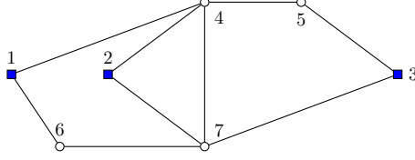
Figure 13: A candidate solution which is infeasible for the MDS DVRP that violates multi-leg PF constraints (12), but does not violate PF constraints (11).
