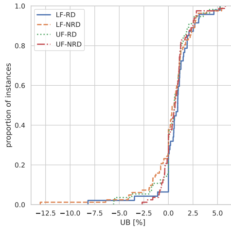
Figure 9: Heuristic solution quality [%] relative to the best known upper bounds for the SDVRP.
