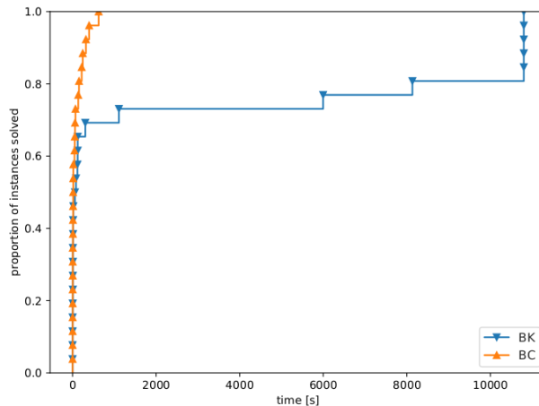
Figure 11: Cumulative proportion of MDTSP instances solved within a given time.
