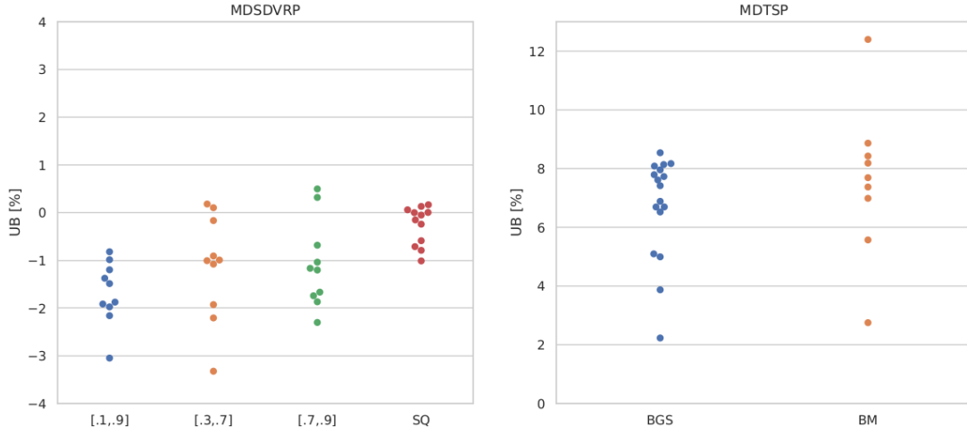
Figure 8: Heuristic solution quality [%] relative to upper bounds of Gulczynski et al. [25] and Bektaş et al. [6] for the MDS DVRP and the MDTSP, respectively.
