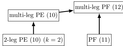
Figure 4: Relations between depot-consistency constraints. An arrow indicates that the set of inequalities at the head dominates the one at the tail.
