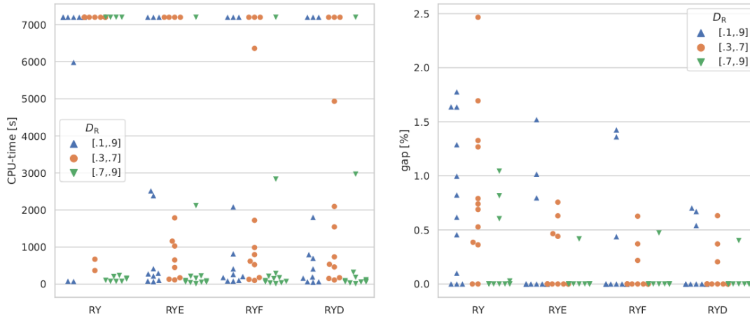
Figure 6: Solution times and optimality gaps of B&C variants for the MDS DVRP on instance set mdsd40 .
