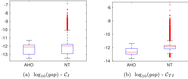
Fig. 4 Temple D: box-plots of the \log_{10} of the complementarity gap gap = X \bullet S using \mathcal{C}_I (plot (a)) and using \mathcal{C}_{TI} (plot (b)).
