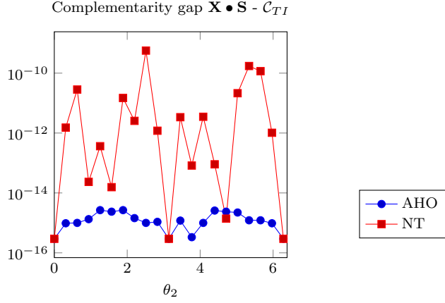
Fig. 5 Parametric D : value of the complementarity gap at the computed solution varying \theta_2 in the definition of D in (54).
