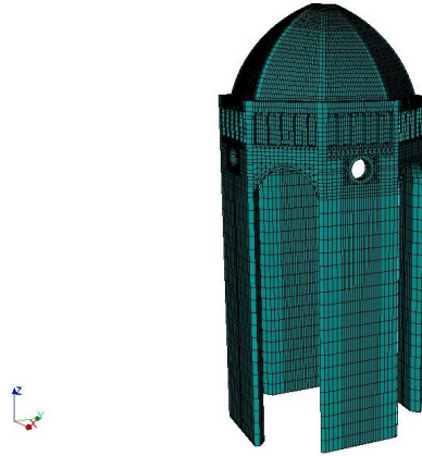
Fig. 1 Finite element model of the domed temple.
