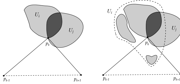
Figure 6: Illustration of the local optimality criteria for path-connected and path-disconnected neighborhoods.
