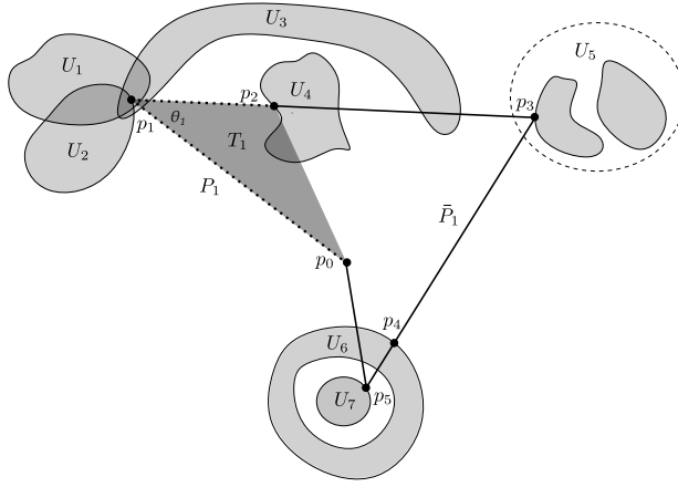
Figure 4: Neighborhood-related objects: T_1 is the shaded triangle (p_0, p_1, p_2) ; \theta_1 is the angle of T_1 at p_1 ; p_2 and p_4 are passing points while the rest are turning points; the dotted path p_0 \rightarrow p_1 \rightarrow p_2 is P_1 ; the complement path denoted by the set of solid line segments is \bar{P}_1 ; \mathcal{U}_1 = \{U_1, U_2\} is the set of active neighborhoods at p_1 . Notice that the binding neighborhood U_3 is not active since it intersects \bar{P}_1 .
