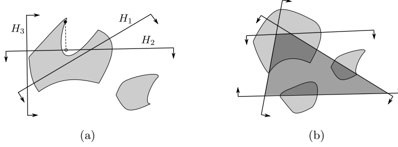
Figure 7: Illustration of projection-closed separators.
