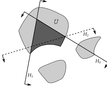
Figure 8: A new BPC separator H_2 that emerges after adding the two separators H_0 and H_1 .
