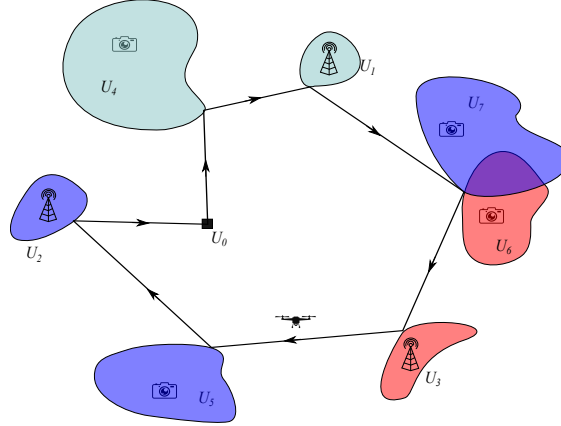
Figure 1: Relay routing for data collection and distribution. Sensors (depicted as cameras) and base stations (depicted as antennas) are each located in one of seven regions. The shape of the regions describes some form of proximity range required for the relay and sensors to exchange data. Irregular shapes may be the result of obstacles and other potential interference sources. Sensors and base stations of the same color indicate to which base station the relay must deliver the data collected by which sensors. The relay is dispatched from its base at location U_0 to conduct the data distribution operation. The closed tour with arrows provides a feasible routing plan.
