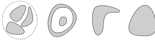
Figure 3: Neighborhoods with different topological properties.
