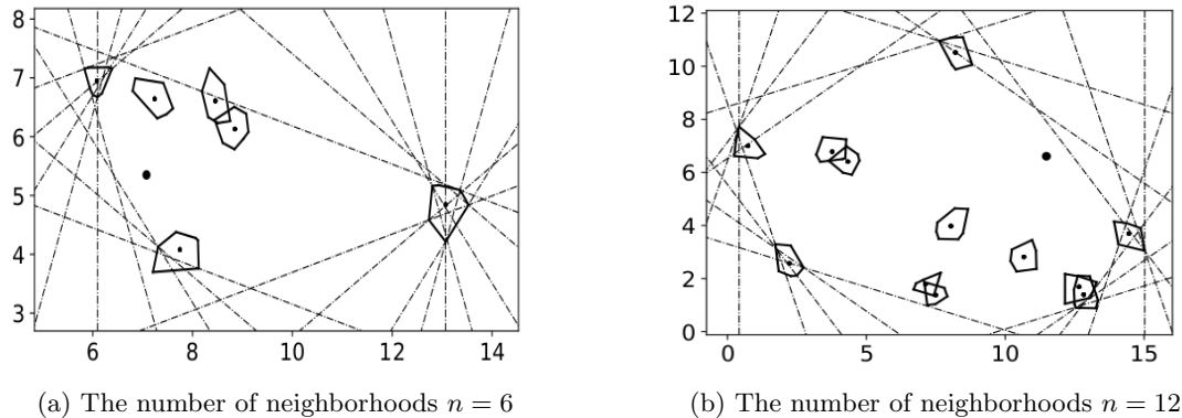
Figure 9: Illustration of separators (dashed lines) generated by Algorithm 1
