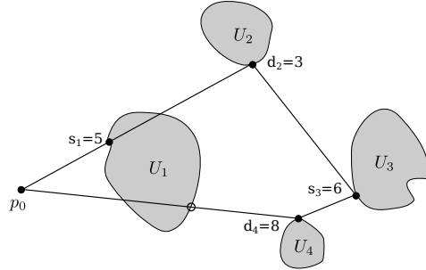
Figure 2: A M-M PDTSPN instance with |I| = 4 neighborhoods and one depot. A feasible tour is constructed by selecting a point (solid black dot) from each neighborhood. In this solution, the vehicle first collects 5 units at neighborhood U_1 , delivers 3 units to U_2 , continues to pick up 6 units at U_3 , then delivers all 8 units to U_4 , before returning to the depot p_0 . Notice that the hollow dot at the boundary of U_1 along with all the subsequent points that intersect that neighborhood are not counted as visits to U_i .
