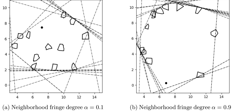
Figure 10: Illustration of separators for problems with convex and non-convex neighborhoods. All the convex neighborhoods are represented by the intersection of half-planes, and the non-convex neighborhoods use the representation introduced in Section 4.3. The fringe degree parameter \alpha controls how close the neighborhoods are to the outskirts of the area. For a small \alpha as in (a), neighborhoods can spread across the area; for a large \alpha as in (b), neighborhoods are located near the area’s periphery.
