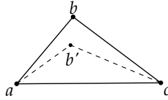
Figure 5: Illustration of Lemma 2.
