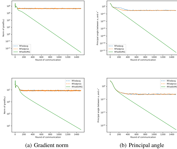
Figure 7: Results for kPCA (3) with MNIST dataset. The data is in \mathbb{R}^{784} ( d = 784 ) and we take r = 5 . The first column is the norm of Riemannian gradient \text{grad } f(x_t) and the second is the principal angle between x_t and the true solution x^* . The two rows corresponds to n = 100 and n = 200 . We take k = n/10 and \tau = 5 for all algorithms.
