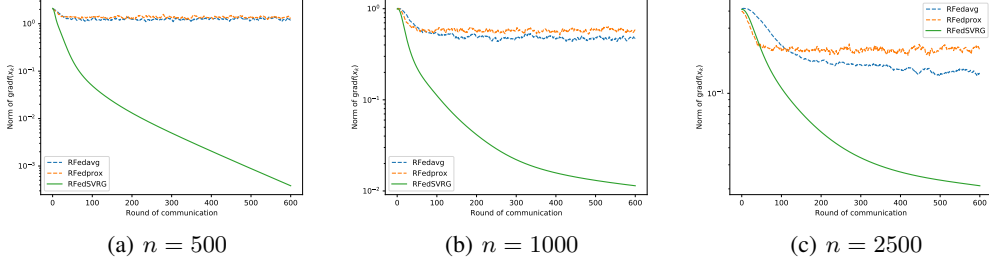
Figure 2: Results for PCA (4). The y-axis denotes \|\text{grad } f(x_t)\| . For each figure, the experiments are repeated and averaged over 10 times.
