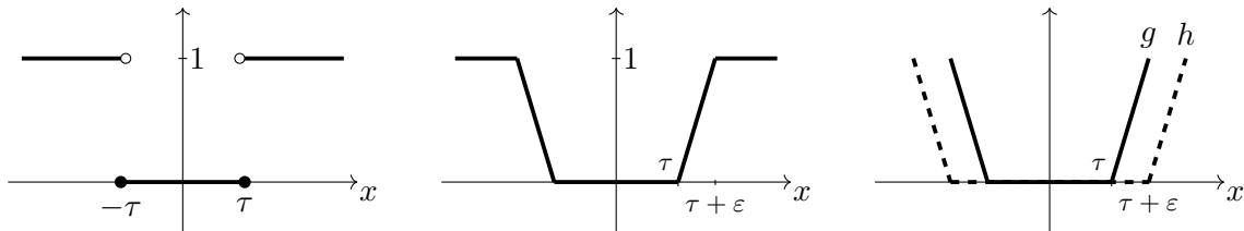
Figure 2: Let \mathbf{x} \in \mathbb{R} . (Left) graph of \|\max(|x| - \tau, 0)\|_0 ; (Center) graph of the approximation function g(x) - h(x) where g(x) = \max\{\frac{1}{\epsilon}(|x| - \tau), 0\} and h(x) = \max\{\frac{1}{\epsilon}(|x| - \tau) - 1, 0\} ; (Right) the DC components of the approximation: g(x) is shown with solid line and h(x) is shown with dashed line.
