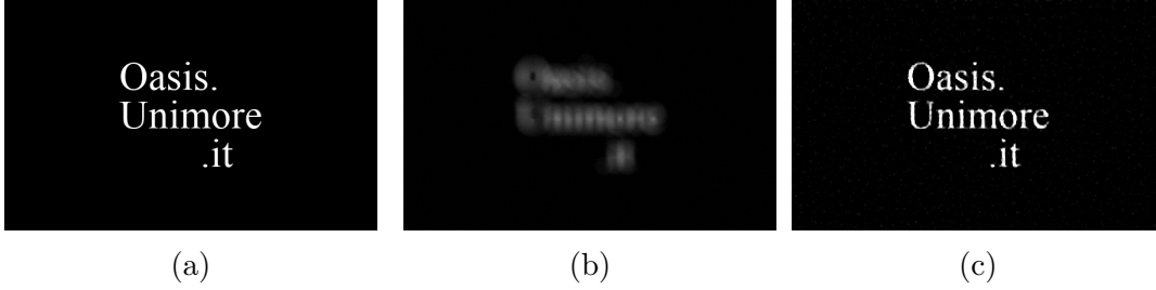
Figure 1: (a) ground truth; (b) blurred sum of the observations; (c) reconstruction obtained by the proposed approach, using the BB rules for the step length selection.
