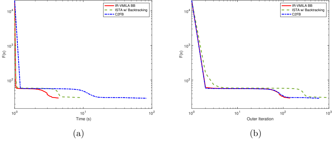
Figure 7: Decrease of the objective function with respect to computational time (left) and outer iterations (right). Comparison between IR-VMILA BB, ISTA with backtracking, and C2FB.
