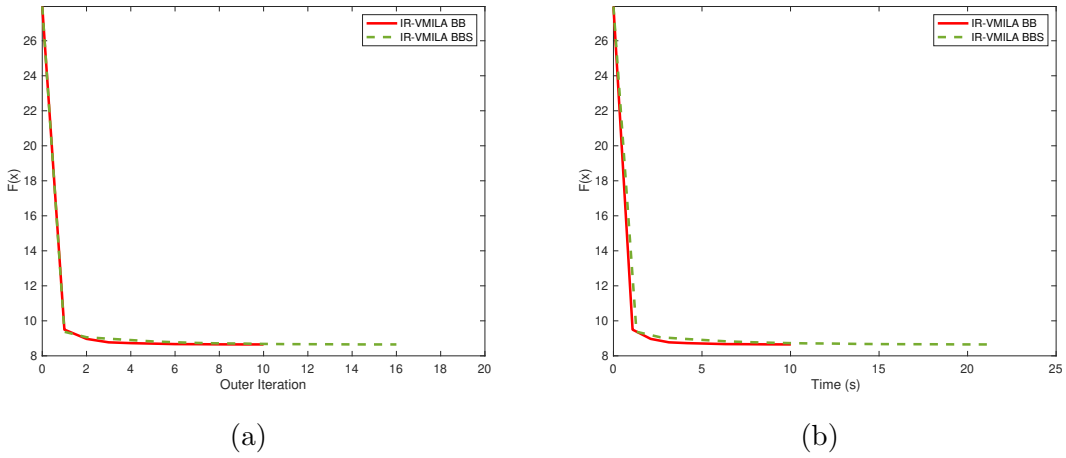
Figure 2: Decrease of the objective function with respect to the outer iterations (left) and computational time (right). Comparison between IR-VMILA equipped with the BB rules, with scaling (BBS) and without scaling (BB).
