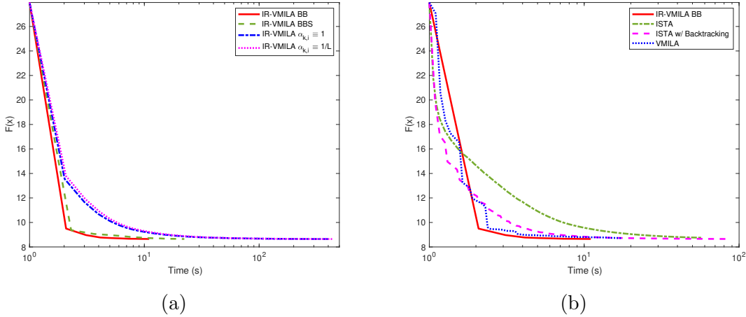
Figure 3: (a) Comparison of several variants of our proposed algorithm: IR-VMILA BB (BB rules, no scaling), IR-VMILA (BB rules, scaling), IR-VMILA \alpha_{k,i} = 1 (constant steplength, no scaling), and IR-VMILA \alpha_{k,i} = 1/L (constant steplength, no scaling); L denotes an estimate of the Lipschitz constant of \nabla f_0 ; (b) comparison between IR-VMILA BB, ISTA, ISTA with backtracking, and VMILAn.
