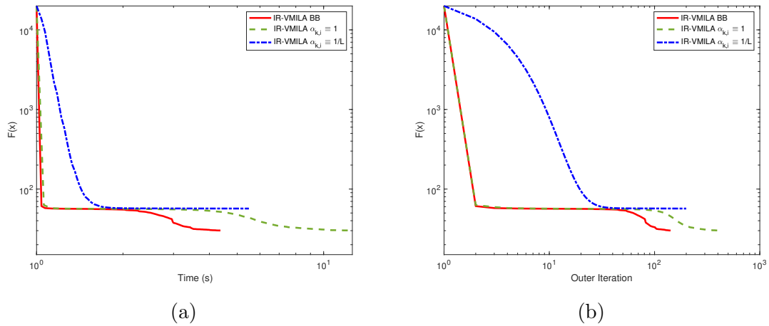
Figure 6: Decrease of the objective function with respect to computational time (left) and outer iterations (right). Comparison between IR-VMILA equipped with the BB rules (no scaling), IR-VMILA with \alpha_{k,i} = 1 , and IR-VMILA with \alpha_{k,i} = 1/L , where L denotes an estimate of the Lipschitz constant of \nabla f_0 .
