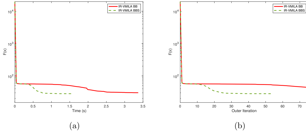
Figure 5: Decrease of the objective function with respect to computational time (left) and the outer iterations (right). Comparison between IR-VMILA equipped with the BB rules, with scaling (BBS) and without scaling (BB).
