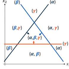
Figure 5: Linear regions defined by the shallow neural network described in Example ?? . Every line corresponds to the activation hyperplane of a different neuron, which is given by \alpha , \beta , and \gamma in parentheses. The arrow next to each line points to the half space in which the inputs activate that neuron. Every linear region has a subset of \{\alpha, \beta, \gamma\} as its corresponding activation set.
