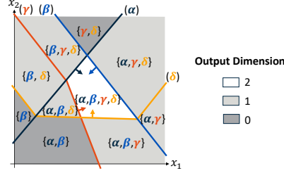
Figure 7: Dimension of the image of the affine function \mathbf{y}_\Pi(\mathbf{x}) associated with each linear region \Pi defined by the neural network described in Example ???. The linear regions are the same illustrated in the third plot of Figure ??.
