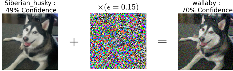
Figure 8: Example of adversarial attack on MobileNetV2 (?). The original image taken by one of the survey authors is classified as ‘siberian_husky,’ but is re-classified as ‘wallaby’ with a small (in an \ell_\infty -norm sense) targeted attack.
