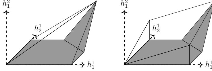
Figure 9: Left: The convex hull of a ReLU neuron (??), and Right: the convex relaxation offered by the big- M formulation (??) Adapted from Anderson et al. ??
