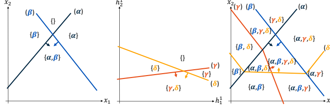
Figure 6: Linear regions defined by the 2 layers of the neural network described in Example ??, following the same notation as in Figure ?. The first and second plots show the linear regions and corresponding activation sets defined by the first and the second layers in terms of their input spaces (the \mathbf{x} and \mathbf{h}^1 spaces). The third plot shows the linear regions defined by the combination of the 2 layers and the union of their activation sets in terms of the input space of the first layer (the \mathbf{x} space).
