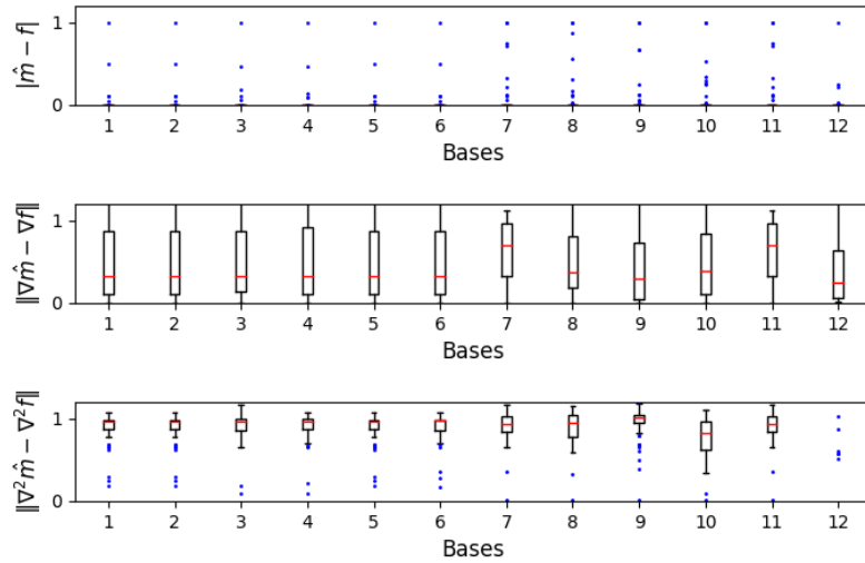
Figure 6: Comparison of |\hat{m} - f| , \|\nabla \hat{m} - \nabla f\| , \|\nabla^2 \hat{m} - \nabla^2 f\| among different bases for the set of 53 problems listed in Table 2 of Appendix A.
