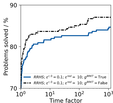
Fig. 9: Time factor performance plot comparing the approach using bracketing ( g^{BRKT}=\text{True} ) against the default of not using it ( g^{BRKT}=\text{False} ). Comparison with tuned hyperparameters of RRHS . Bracketing does not improve performance.
