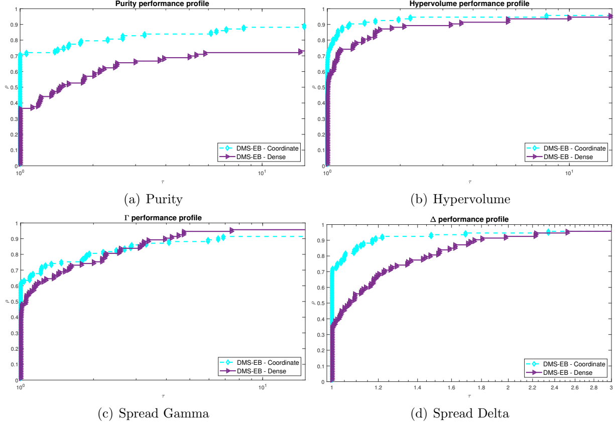
Figure 2: Performance profiles for DMS considering different types of positive spanning sets and a maximum budget of 5000 function evaluations.
