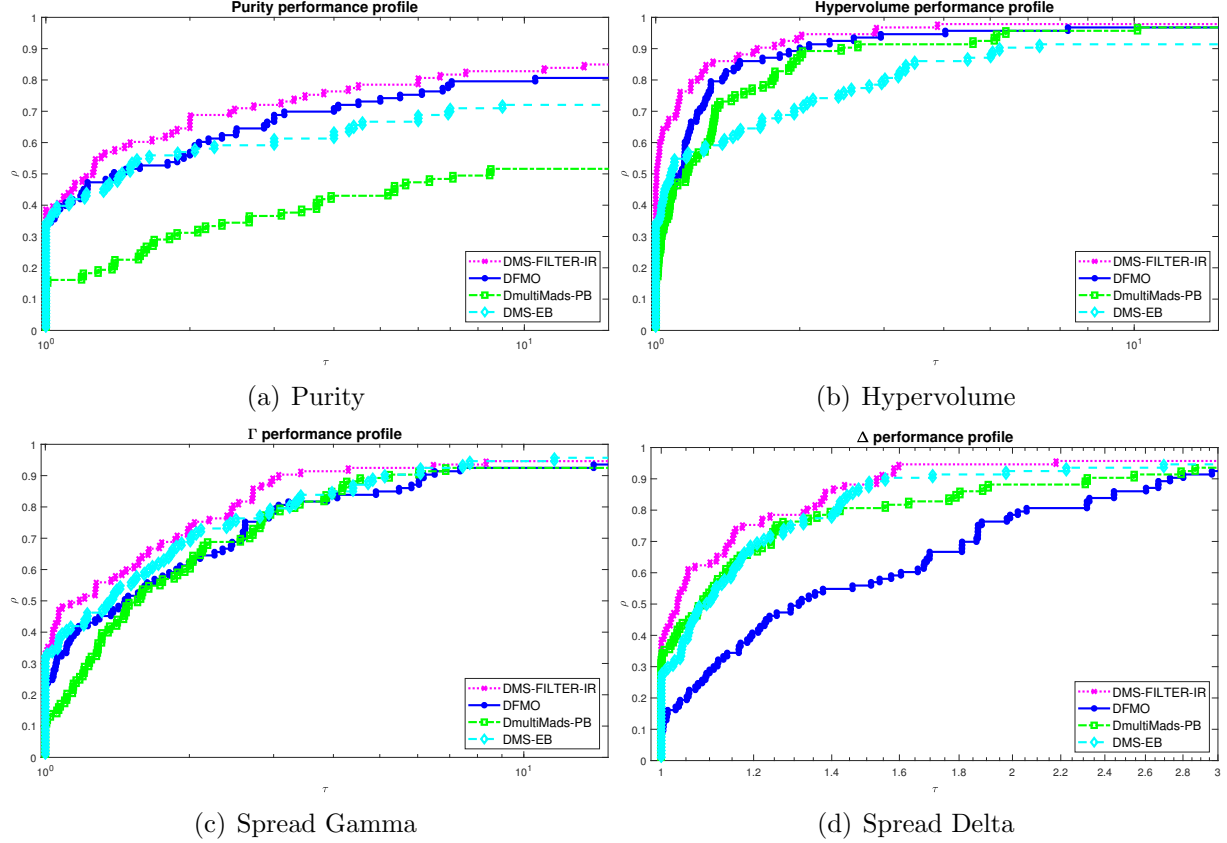
Figure 4: Comparing DMS-FILTER-IR with DFMO, DMultiMADS-PB, and DMS based on performance profiles for a maximum of 500 function evaluations.
