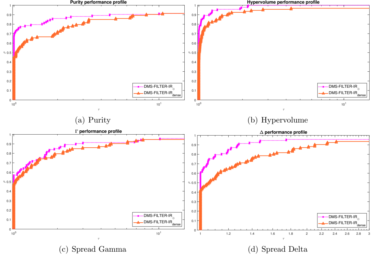
Figure 3: Performance profiles for DMS-FILTER-IR considering different types of positive spanning sets and a maximum budget of 5000 function evaluations.
