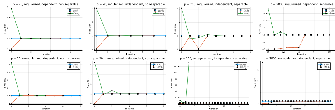
Figure 2: Step size chosen on each iteration for the plots in Figure 1. For iterations where the hybrid method took a gradient step, the gradient descent step size is shown (where a pure Newton step was taken the step size is 1).
