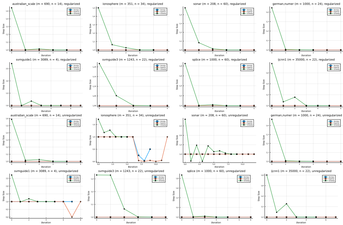
Figure 4: Step sizes of methods on real logistic regression datasets, in 8 cases where we observed typical performance.
