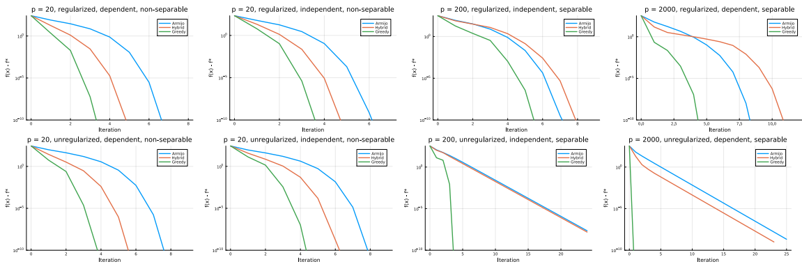
Figure 1: Comparison of Newton with Armijo backtracking, hybrid gradient-Newton, and greedy Newton on logistic regression problems with regularization (top row) and without regularization (bottom row). From left to right, in the bottom row the problems are convex, strongly-convex, strictly-convex, and convex (all problems in the top row are strongly-convex). The right two datasets are linearly separable and the left two datasets are non-separable.
