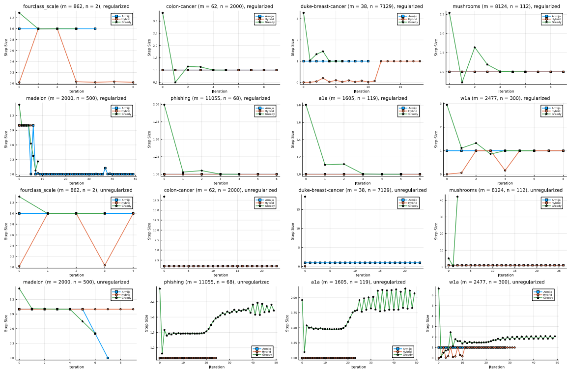
Figure 6: Step sizes of methods on real logistic regression datasets, in 8 cases where we observed atypical performance in either the regularized or unregularized setting.
