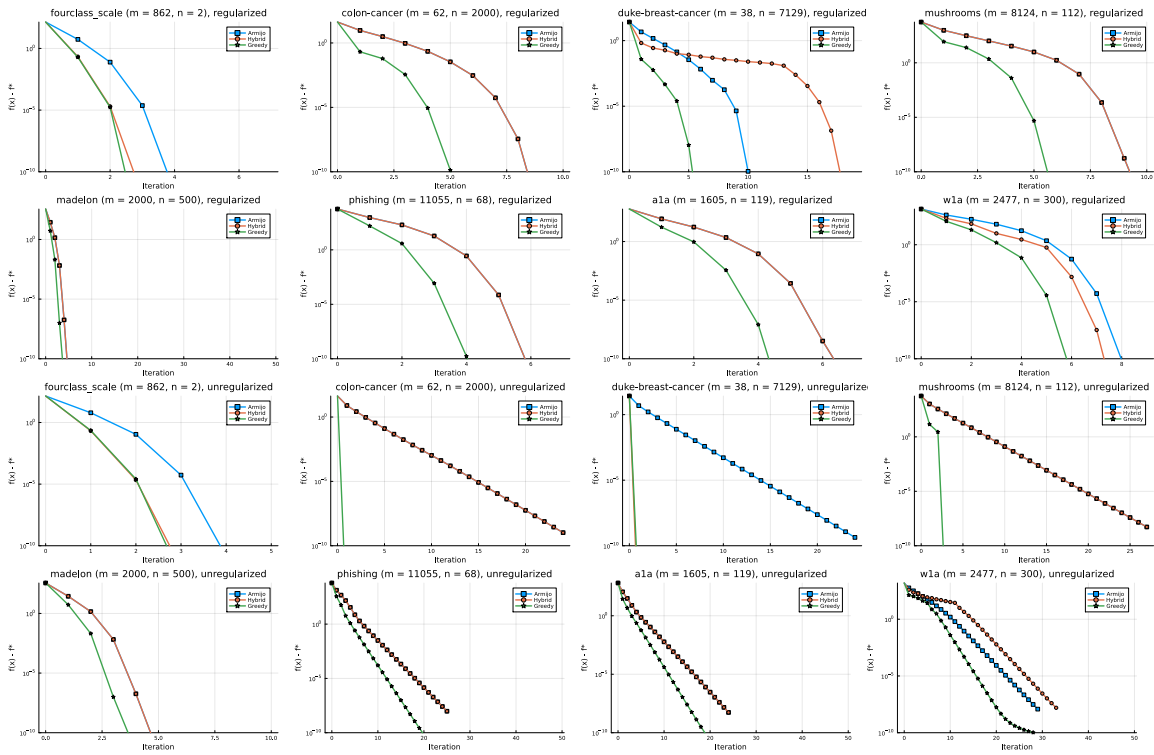
Figure 5: Comparison of methods on real logistic regression datasets, in 8 cases where we observed atypical performance in either the regularized or unregularized setting.
