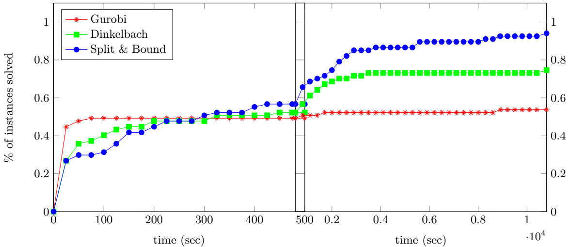
Figure 3: Performance comparison of the exact algorithms. Note the different scale on the x -axis: the plot on the left displays the time range from 0 to 500 seconds, the plot on the right from 500 seconds to 3 hours.
