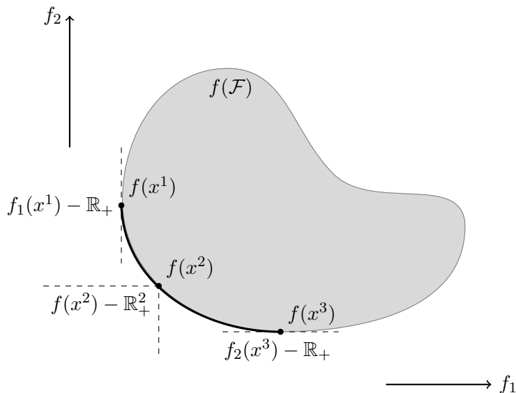
Figure 1: Image set of a bi-objective instance.
