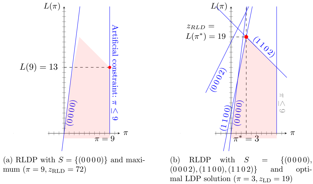
Figure 5.4: Lagrangian Dual Problem and sequence of Restricted Lagrangian Dual Problems
