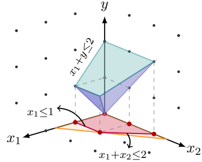
(d) Projection of the resulting polyhedron matches \text{Conv}(X)
