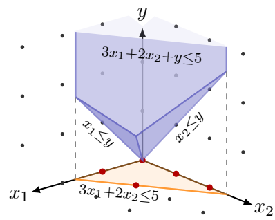
(b) Extended polyhedron P' and its projection P
