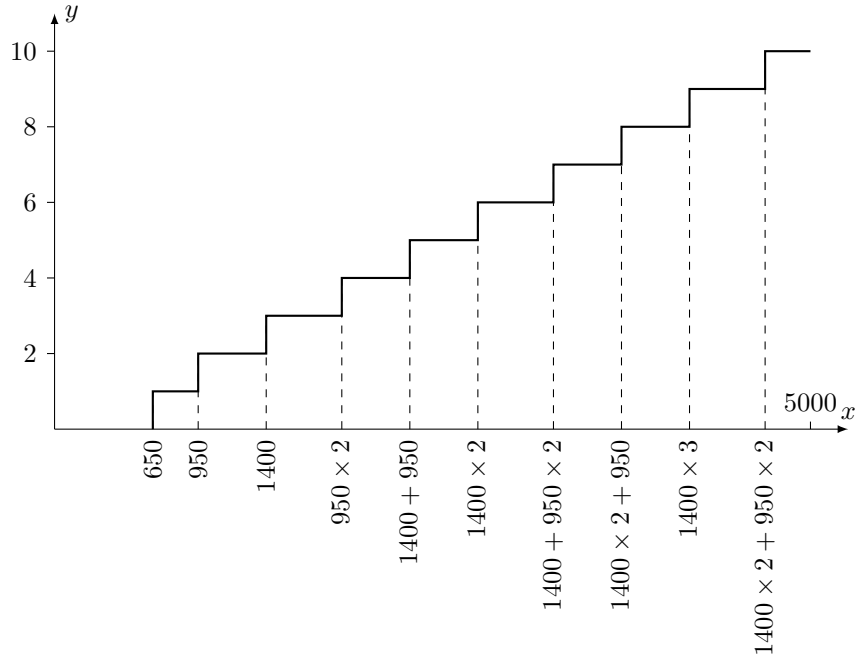
Figure 4.13: An optimal “Scale of Indices”.
