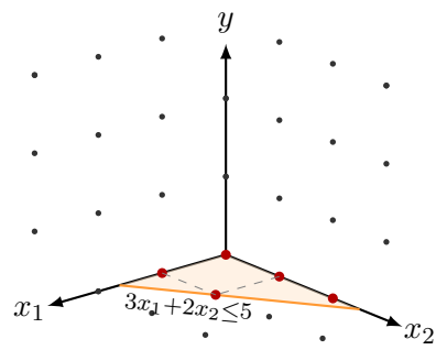
(a) Polyhedron P
