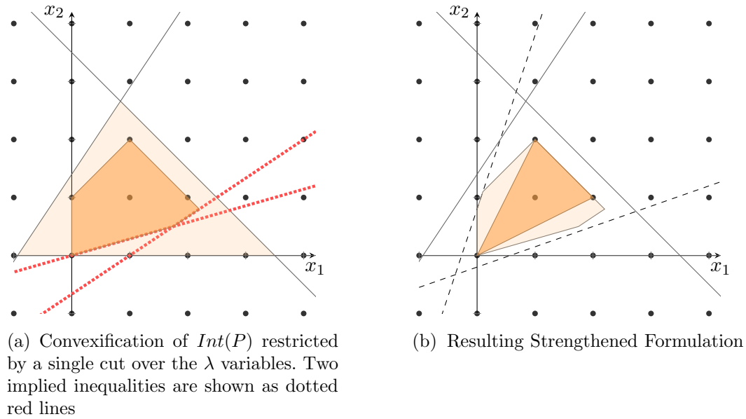
Figure 4.4: Effect of a cut over the generated variables
