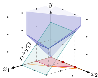
(c) Insertion of cut x_1 + y \leq 2 over polyhedron P'
