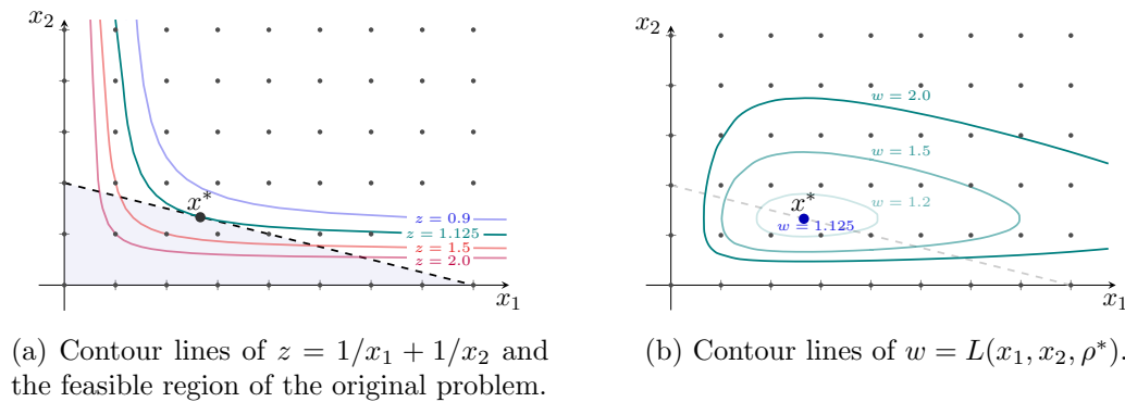
Figure 5.1: The effect of dualizing the constraint x_1 + 4x_2 \leq 8 in (5.4) with multiplier \rho^* = 9/64
