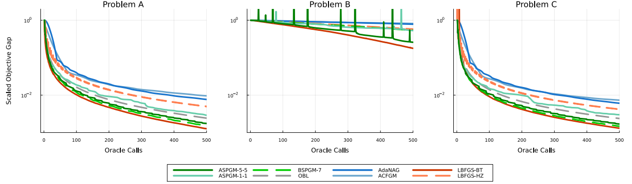
Figure 5: Performance on poorly conditioned problem instances with d = 1000 , as measured by (f(x_n) - f_\star)/(f(x_0) - f_\star) .
