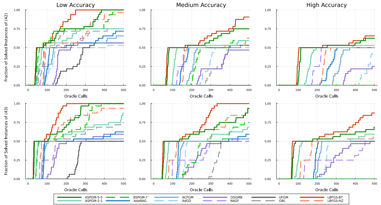
Figure 9: Performance comparison for locally smooth problems (4.5) and (4.6). The performance is measured by (f(x_n) - f_\star)/(f(x_0) - f_\star) and the target accuracies from left to right are 10^{-4} , 10^{-7} , 10^{-10} .
