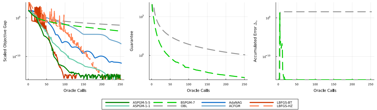
Figure 3: Performance data from logistic regression (4.2) run on the colon-cancer dataset. On the left, we show the alternate performance measure (f(x_n) - f_*)/(\frac{1}{2}\|x_0 - x_*\|^2) . In the middle plot, we compare the guarantees of BSPGM-7 and OBL (ignoring error terms). This corresponds to L_n/\tau_n . The right plot shows the accumulated error \Delta_n for BSPGM-7 and OBL.
