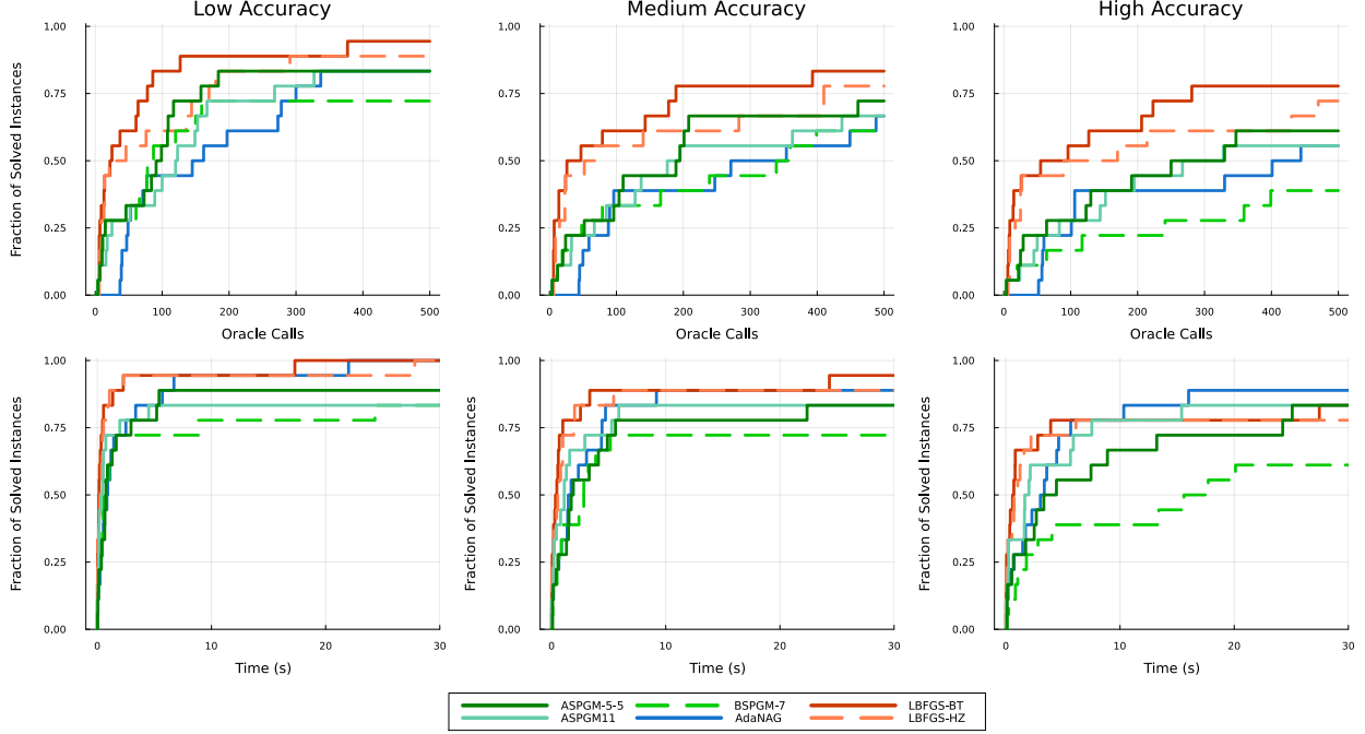
Figure 4: Performance results for feasibility problems over LP instances from [52]. The performance is measured by (f(x_n) - f_\star)/(f(x_0) - f_\star) and the target accuracies from left to right are 10^{-4} , 10^{-7} , 10^{-10} .
