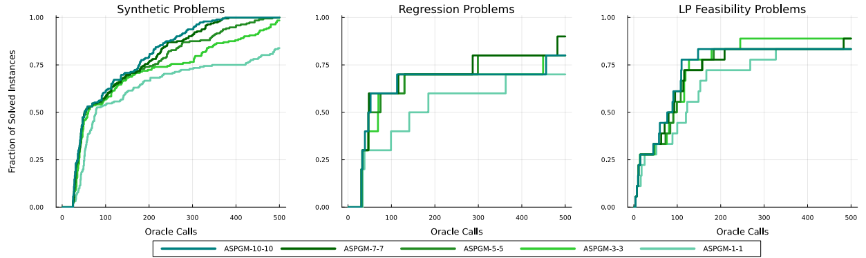
Figure 6: Performance comparison of ASPGM with different memory sizes. From left to right, we show results with performance measured by (f(x_n) - f_\star)/(f(x_0) - f_\star) at accuracy 10^{-7} , for synthetic problems, regression problems, and LP feasibility problems.
