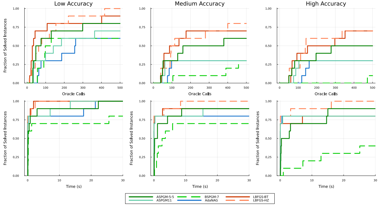
Figure 2: Performance results for least squares regression (4.1) and logistic regression (4.2) problems from LIBSVM [51]. The performance is measured by (f(x_n) - f_*)/(f(x_0) - f_*) and the target accuracies from left to right are 10^{-4}, 10^{-7}, 10^{-10} .
