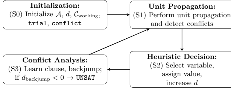
Figure 4: A simplified overview of the generic CDCL ( [19, Algorithm 10]) solving cycle using the parameters: \mathcal{A} (current partial assignment), d (decision level), \mathcal{C}_{\text{working}} (working clause set), \text{trial} (assignment record), \text{conflict} (conflict flag), and d_{\text{backjump}} (backjump level). (S1)–(S3) repeat until \mathcal{C}_{\text{working}} = \emptyset
