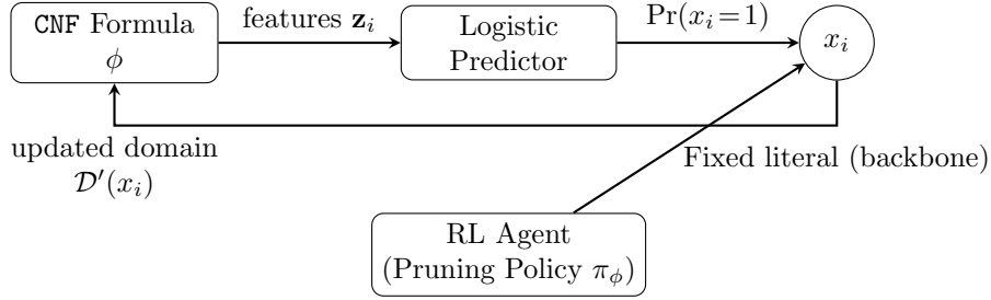
Figure 5: ML-enhanced propagation: the logistic model predicts backbone literals, while an RL agent prunes infeasible branches to accelerate propagation.
