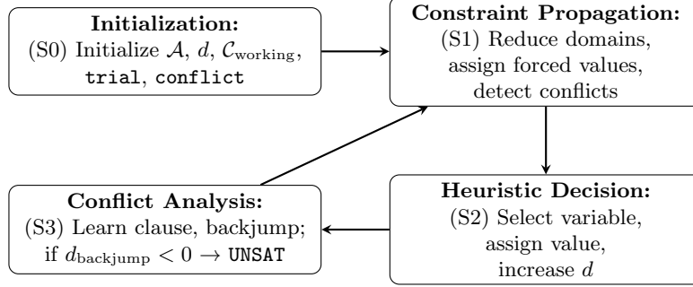
Figure 3: A simplified overview of the generic LCG ( [19, Algorithm 9]) solving cycle using the parameters: \mathcal{A} (current partial assignment), d (decision level), \mathcal{C}_{\text{working}} (working constraint set), \text{trial} (assignment record), \text{conflict} (conflict flag), and d_{\text{backjump}} (backjump level). (S1)–(S3) repeat until all constraints in \mathcal{C}_{\text{working}} are satisfied or a root-level conflict is detected.
