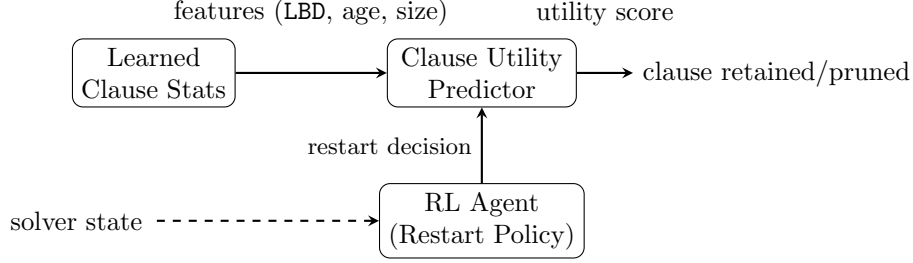
Figure 7: Conflict analysis enhanced by ML-based clause evaluation and RL-guided restart scheduling. LBD (Literal Block Distance) is a metric for evaluating clause quality during conflict learning that is discussed in [19, Section 3.2].
