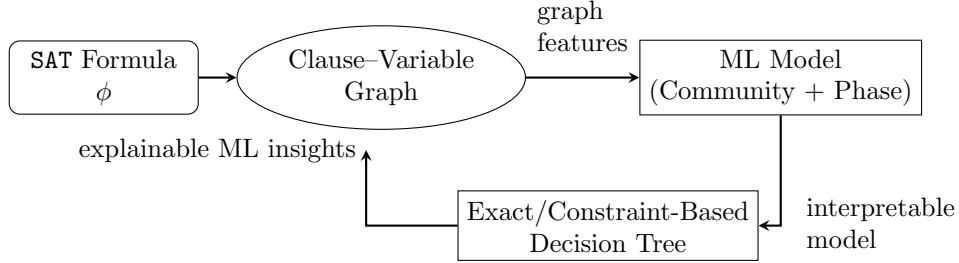
Figure 8: Beyond the solving loop: ML models extract community structure and support interpretable decision-tree learning through exact and constraint-based formulations.
