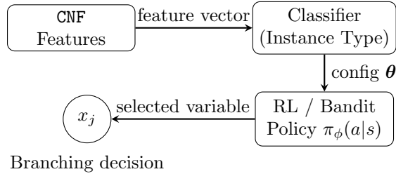
Figure 6: Adaptive branching via ML classification and RL/bandit decision policies. The model selects the next variable and polarity based on learned solver statistics.
