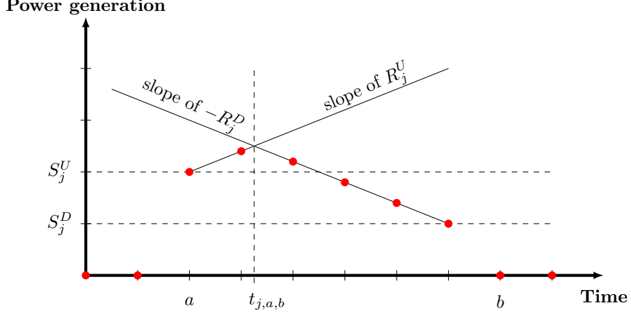
Fig. 2 Definition of t_{j,a,b} . Red points indicate the maximum power generation at each time step when \gamma_{j,a,b} = 1 .
