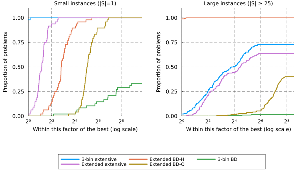
Fig. 3 Performance profiles comparing solution approaches on the IEEE 118-bus instance and SMS++ instances with 10, 50, and 100 thermal units.
