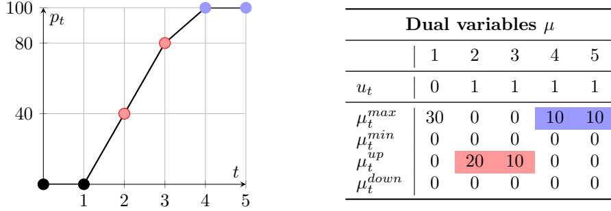
Fig. D1 Optimal dual multipliers \mu and the corresponding power generation trajectory when the unit is on from time 2 to time 5. Blue: maximum generation constraint active, red: ramp-up constraint active.
