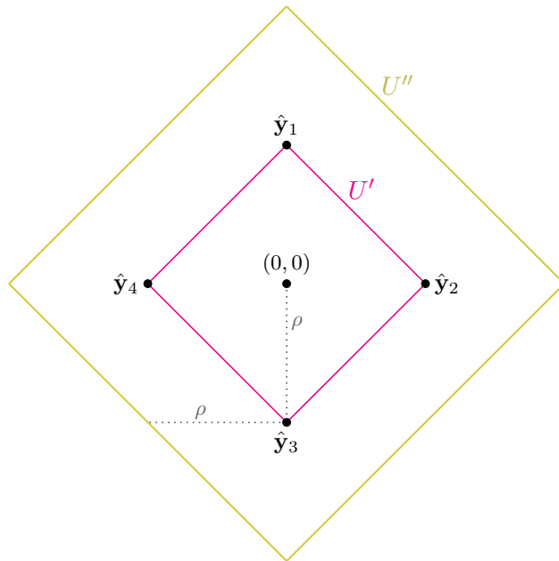
Figure A1: Illustration for proof of Proposition 1 with boundaries of U' and U'' marked
