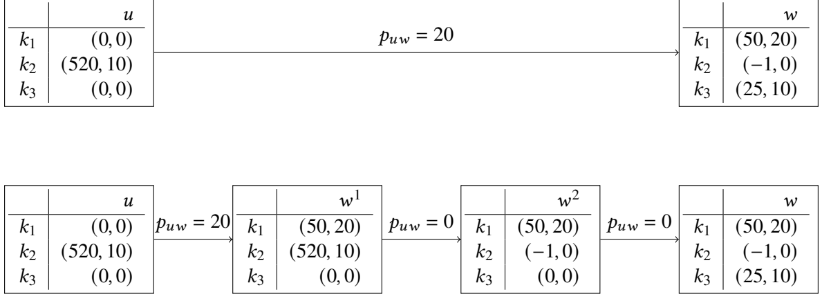
Figure 3: Arc-splitting in a multi-leg trajectory graph. An arc from node u to node w (top) and its splitting into three arcs: u \rightarrow w^1 , w^1 \rightarrow w^2 , w^2 \rightarrow w (bottom).
