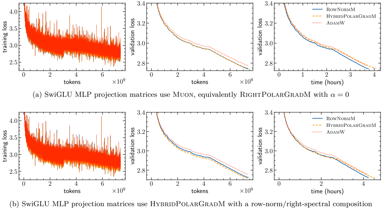
Figure 1: Training and validation losses for Gemma 3 1B-style pre-training. In each subfigure, configurations (i)–(iii) differ only in the optimizer assigned to the input embedding and LM head matrices: ROWNORMM, HYBRIDPOLARGRADM, or ADAMW.
