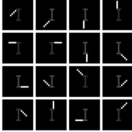
Fig. 4: Basis images with sparsity s = 132 of the swimmer dataset obtained after applying ARBPG.
