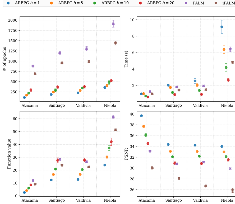
Fig. 1: Performance comparison of the evaluated algorithms across four test images (“Atacama”, “Santiago”, “Valdivia”, and “Niebla”) over ten randomly generated seeds. The panels display the average number of epochs, computational time in seconds, final function values, and PSNR. The error bars denote the standard deviation across the ten independent runs.
