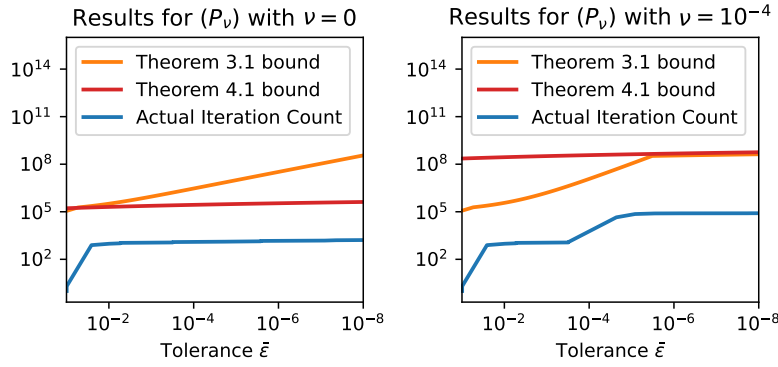
FIGURE 6. Plots of the guaranteed bounds on the number of iterations of rPDHG and the actual number of iterations of rPDHG for the LP instance (P_\nu) for \nu = 0 (left) and \nu = 10^{-4} (right).
