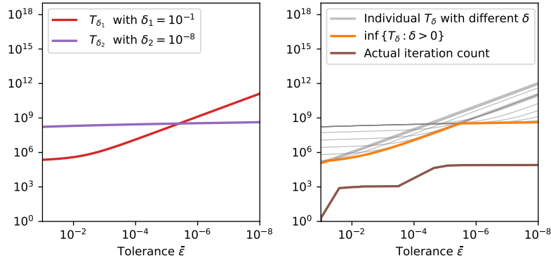
FIGURE 5. (Left) Plots of T_\delta for \delta = 10^{-1} and \delta = 10^{-8} , as a function of the required tolerance \bar{\varepsilon} = \varepsilon_{\text{cons}} = \varepsilon_{\text{gap}} for the linear optimization instance (P_\nu) with \nu = 10^{-4} . (Right) Plots of the actual iteration counts of rPDHG, and the lower envelope \inf_{\delta > 0} T_\delta .
