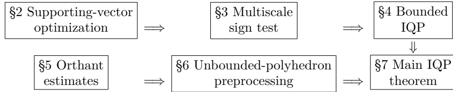
Figure 1: Dependencies among the principal internal results used to prove Theorem 1.1. Each arrow points from a component to a later result that uses it; cited external routines are omitted.
