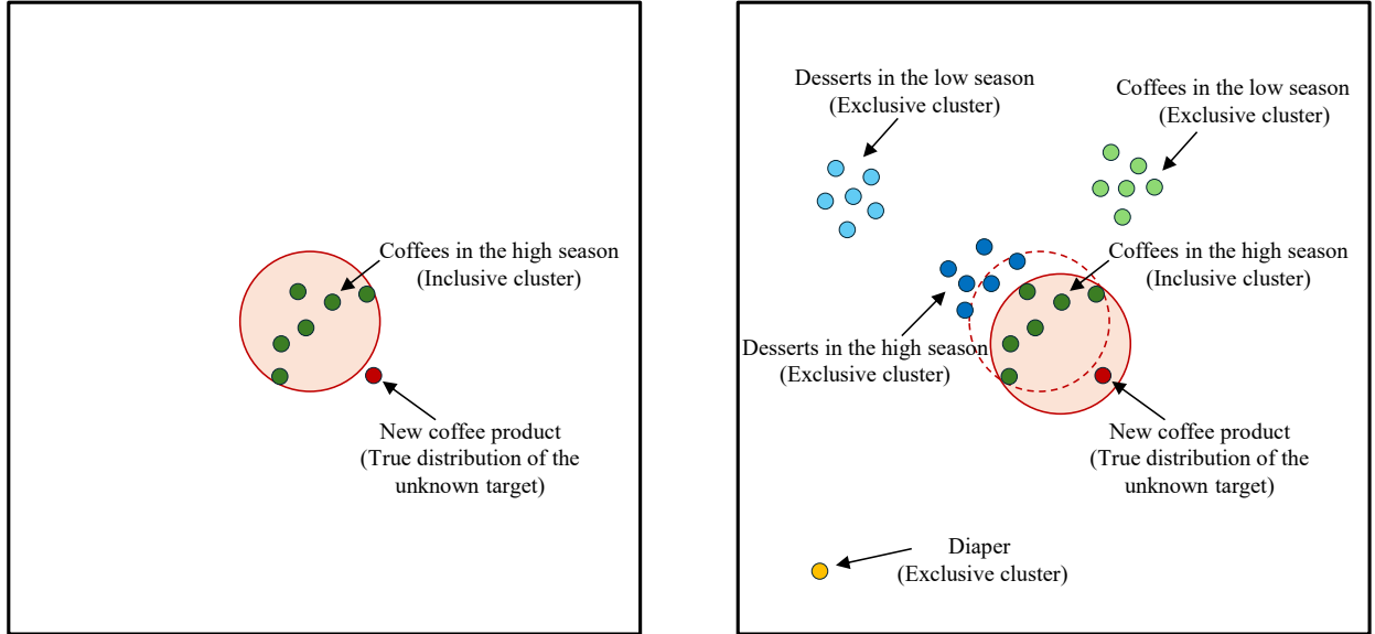
(a) Inclusive clusters alone: a ball that merely encloses them can leave the target distribution outside.
