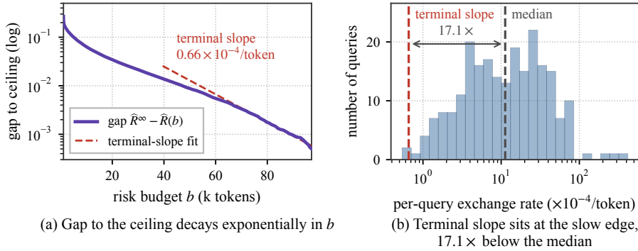
Figure 9: The large-budget law against the data on Llama-3.2-3B, with the protocol of Figure 3. The terminal slope is 0.66 \times 10^{-4} per risk-adjusted token, 17.1\times below the median of the fitted exchange rates.
