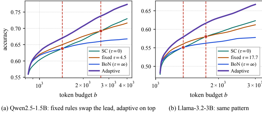
Figure 2: Fixed-voting frontiers cross, while the adaptive frontier dominates ((a) Qwen2.5-1.5B, (b) Llama-3.2-3B; MATH-500; protocol in Appendix A.5). Each panel shows four frontiers: SC ( \tau = 0 ), BoN ( \tau = \infty ), the intermediate fixed temperature, and the adaptive voting policy. Red dots with dashed guides mark the budgets where the accuracy lead between two fixed-voting rules swaps
