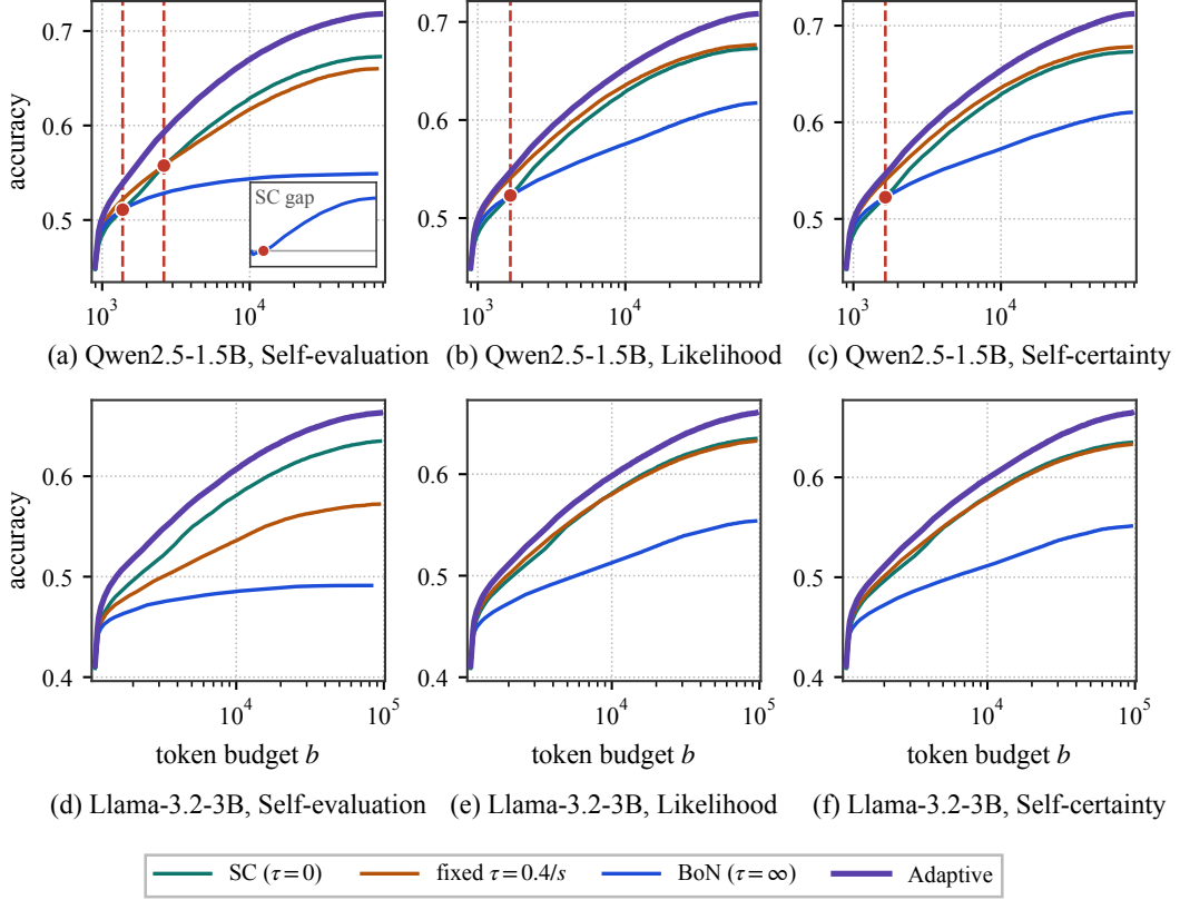
Figure 7: Figure 2 on the full MATH-500 population, with the Likelihood and Self-certainty scores added; panels (a)–(c) Qwen2.5-1.5B, (d)–(f) Llama-3.2-3B. Red dots mark the budgets at which the lead among the fixed rules swaps, and the inset in panel (a) shows the pairwise gap of SC over each competitor crossing zero. On the full Llama-3.2-3B population BoN leads SC only marginally at the smallest budgets, so panels (d)–(f) carry no markers.
