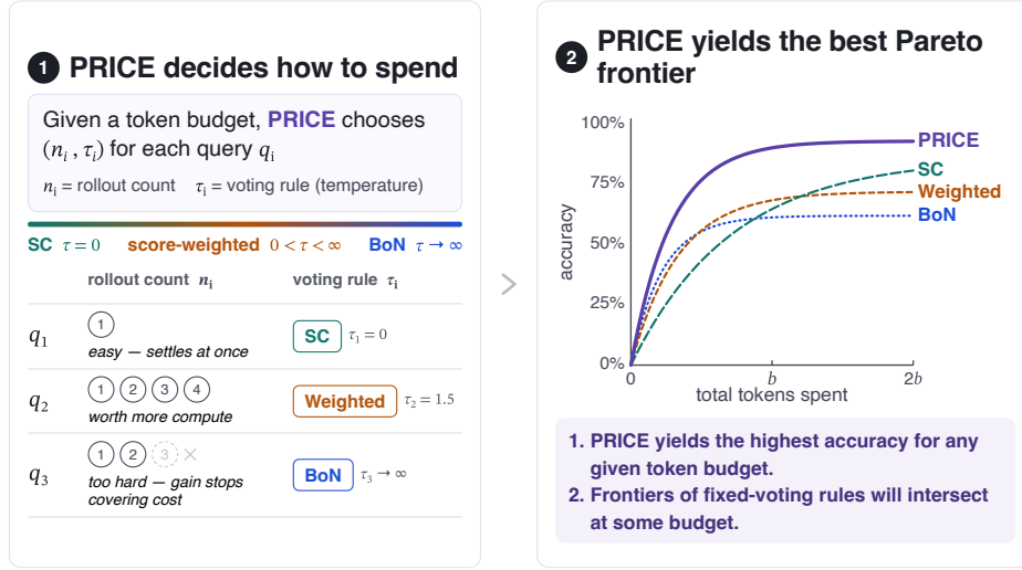
Figure 1: Illustration of the proposed PRICE method.
