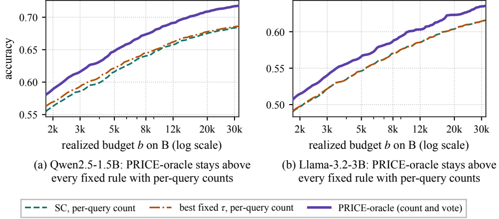
Figure 6: Split-pool frontiers of PRICE-oracle with the self-evaluation score ((a) Qwen2.5-1.5B, (b) Llama-3.2-3B). PRICE-oracle, the best global temperature and SC all choose per-query counts from the A primitives and are evaluated with the actual B token sums. The best global temperature is selected at each budget after seeing the results, so the orange curve is an envelope over fixed rules rather than a single policy.
