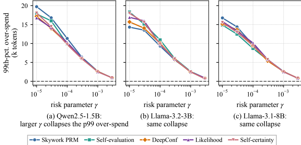
Figure 8: Empirical overspend relative to the risk budget ((a) Qwen2.5-1.5B, (b) Llama-3.2-3B, (c) Llama-3.1-8B; shared y range): p99 over-spend beyond b vs. \gamma at matched work ( \bar{n} \approx 8 per \gamma ), five scores. 99% of queries spend at most b plus the value shown; the dashed gray line marks zero over-spend, and the collapse is uniform across scores and generators.
