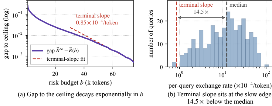
Figure 3: The large-budget law against the data (PRICE-oracle, Qwen2.5-1.5B). (a) The gap to the accuracy ceiling decays almost linearly on the log scale when the budget is large, and the red dashed line is the terminal-slope fit over the upper quarter of the budget range. (b) The terminal slope sits at the slow edge of the per-query exchange rates (18) fitted on the solvable queries.
