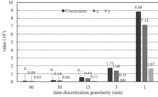
Figure 1 Impact of time discretization on SSND( \mathcal{D}_T^\Delta, \mathcal{K} ) model size.
