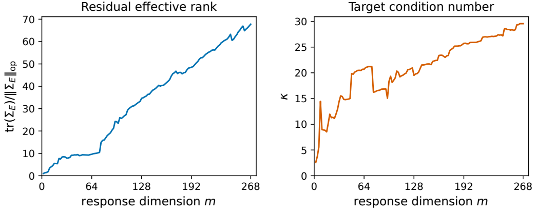
Figure 4: Effective rank \text{tr}(\Sigma_E^{P_m}) / \|\Sigma_E^{P_m}\|_{\text{op}} and condition number \kappa_{P_m} of the target law P_m in our CESNET experiment, as a function of the response dimension m .
