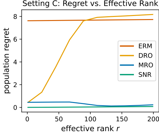
Figure 2: Target population regret R(\hat{\mathbf{A}}[P_{s,n}], P_r) for Setting C, as a function of the target residual effective rank r = r_{\text{eff}}(\Sigma_E^{P_r}) .
