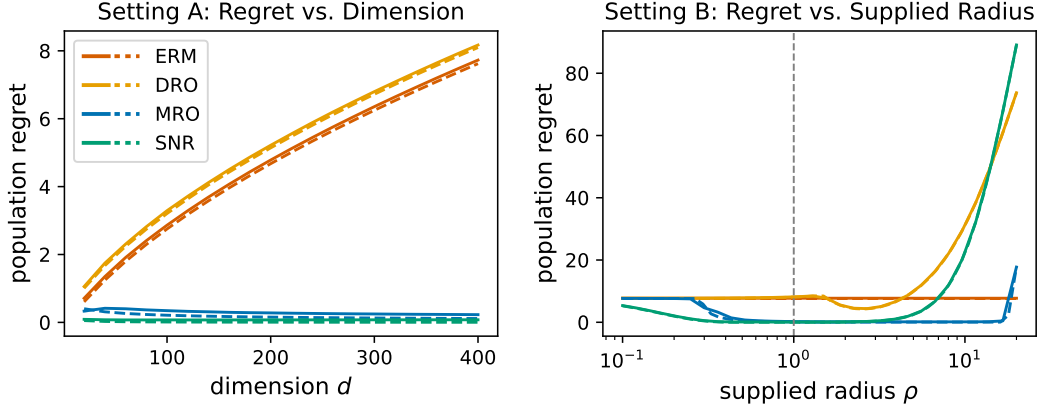
Figure 1: Target population regret R(\hat{\mathbf{A}}[P_{s,n}], P) for Settings A (left) and B (right). Solid curves show finite-sample averages, while dashed curves show population benchmarks. For Setting B, the dashed vertical line marks the corruption budget \varepsilon = 1 .
