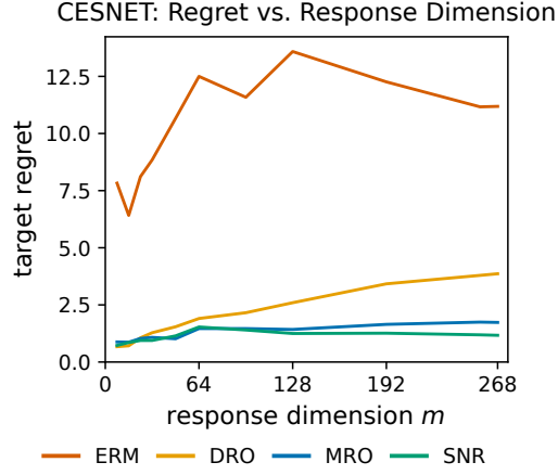
Figure 3: Target regret R(\hat{\mathbf{A}}[\tilde{P}_m], P_m) for our CESNET experiment, as a function of the response dimension m .
