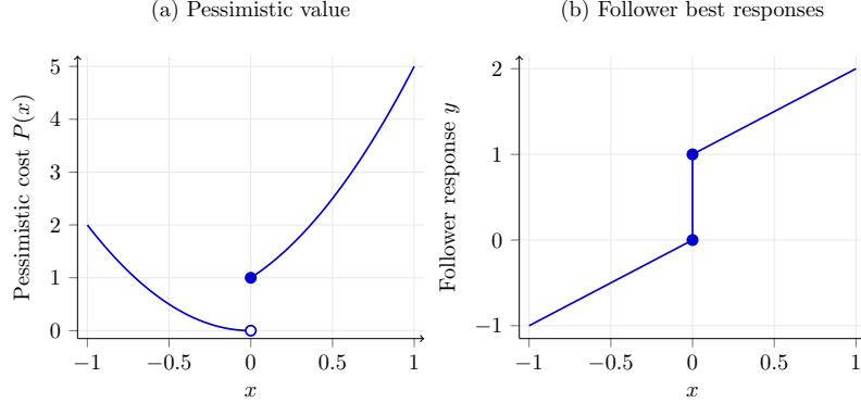
FIGURE 2. Pessimistic cost and follower best responses in the modified Dempe example. Left: The open circle marks the unattained limiting cost and the solid circle marks the actual cost at indifference. Right: The vertical segment is the full best-response set S(0) = [0, 1] .
