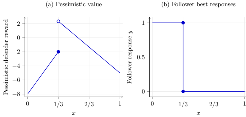
FIGURE 1. Pessimistic defender reward and follower best responses in the security game example. Left: The open circle marks the unattained limiting reward and the solid circle marks the actual reward at indifference. Right: The vertical segment is the full best-response set S(1/3) = [0, 1] .
